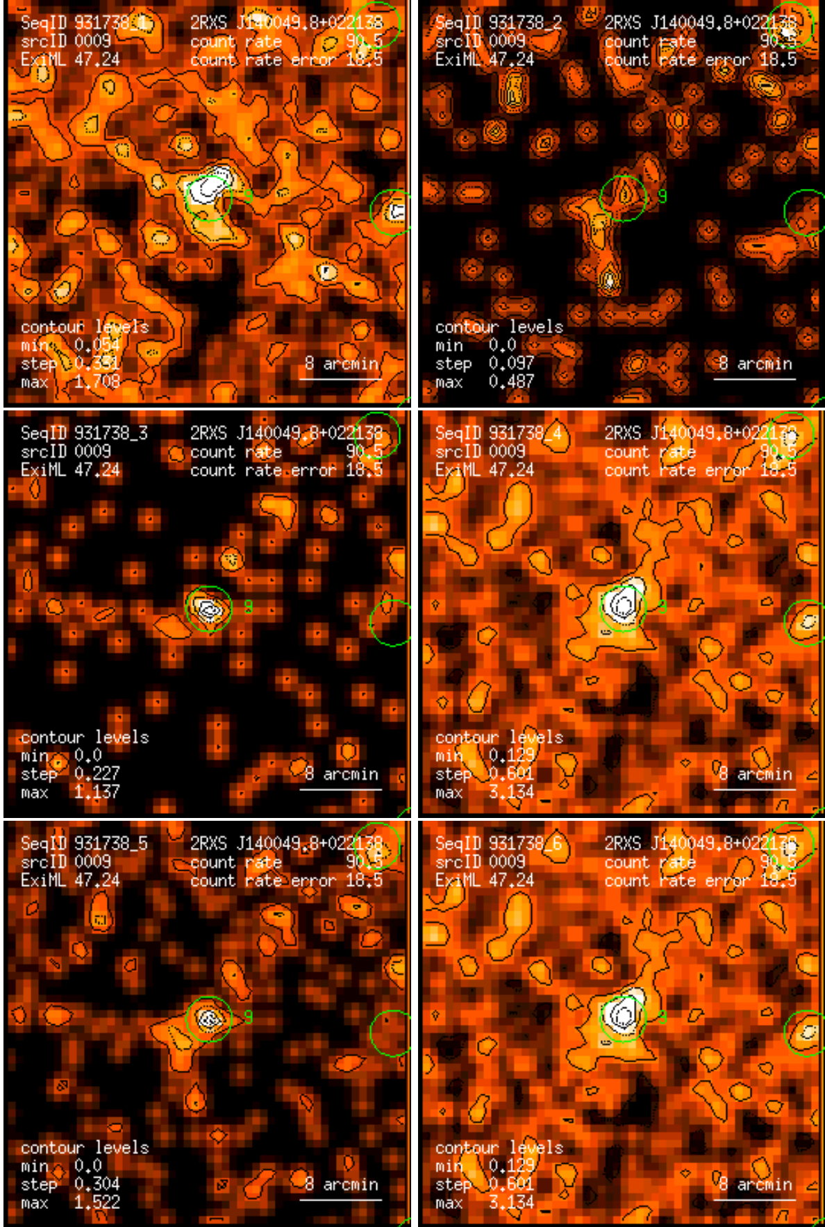
Figure 9: RASS 931738: detection 0009: band rate images, Gaussian filter: (1) PSPC channels 11 – 41, (2) 52 – 90, (3) 91 – 201, (4) 11 – 235, (5) 52 – 201, (6) 11 – 201. Broad band rates in counts/ks. Band rate contour levels in counts/ks/arcmin 2 .
