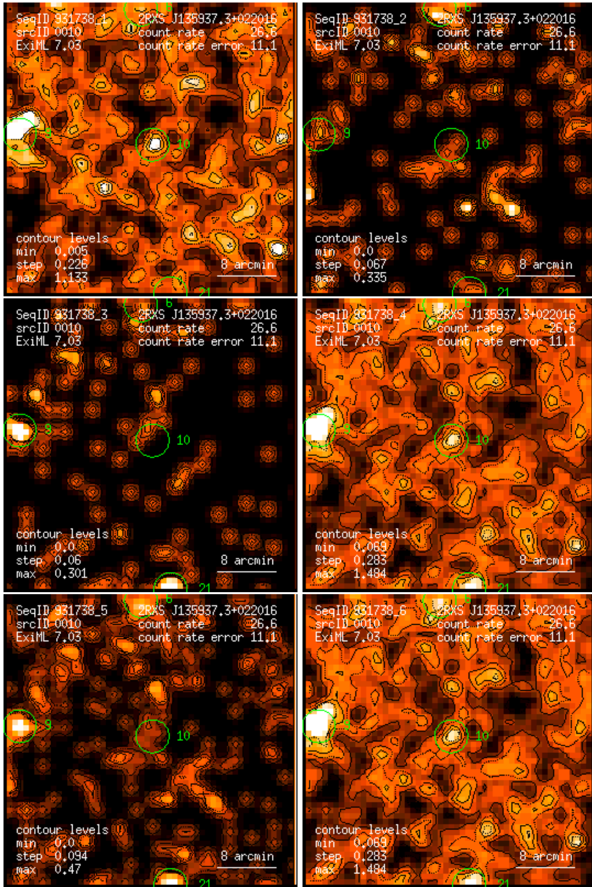
Figure 10: RASS 931738: detection 0010: band rate images, Gaussian filter: (1) PSPC channels 11 – 41, (2) 52 – 90, (3) 91 – 201, (4) 11 – 235, (5) 52 – 201, (6) 11 – 201. Broad band rates in counts/ks. Band rate contour levels in counts/ks/arcmin 2 .
