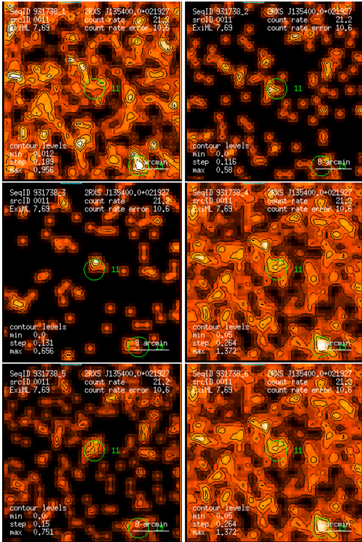
Figure 11: RASS 931738: detection 0011: band rate images, Gaussian filter: (1) PSPC channels 11 – 41, (2) 52 – 90, (3) 91 – 201, (4) 11 – 235, (5) 52 – 201, (6) 11 – 201. Broad band rates in counts/ks. Band rate contour levels in counts/ks/arcmin 2 .
