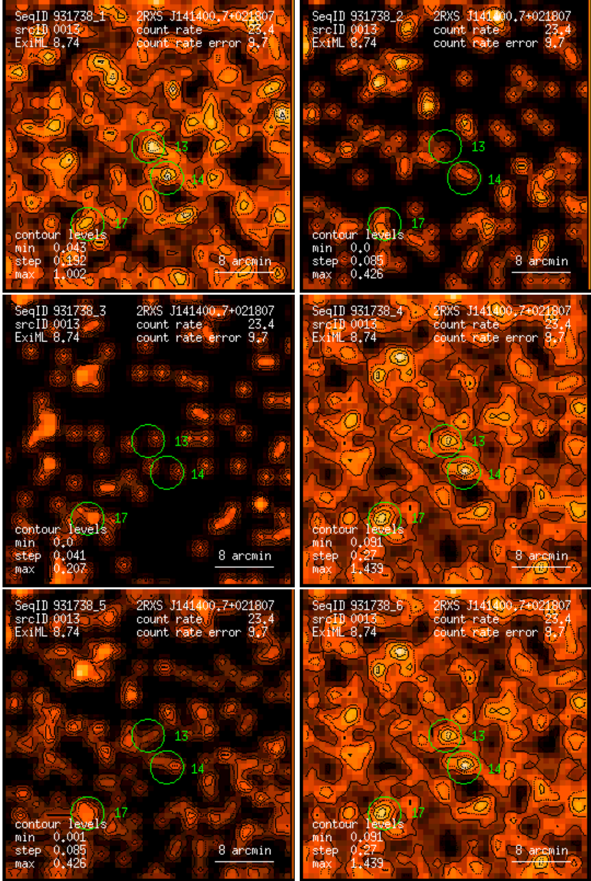
Figure 13: RASS 931738: detection 0013: band rate images, Gaussian filter: (1) PSPC channels 11 – 41, (2) 52 – 90, (3) 91 – 201, (4) 11 – 235, (5) 52 – 201, (6) 11 – 201. Broad band rates in counts/ks. Band rate contour levels in counts/ks/arcmin 2 .
