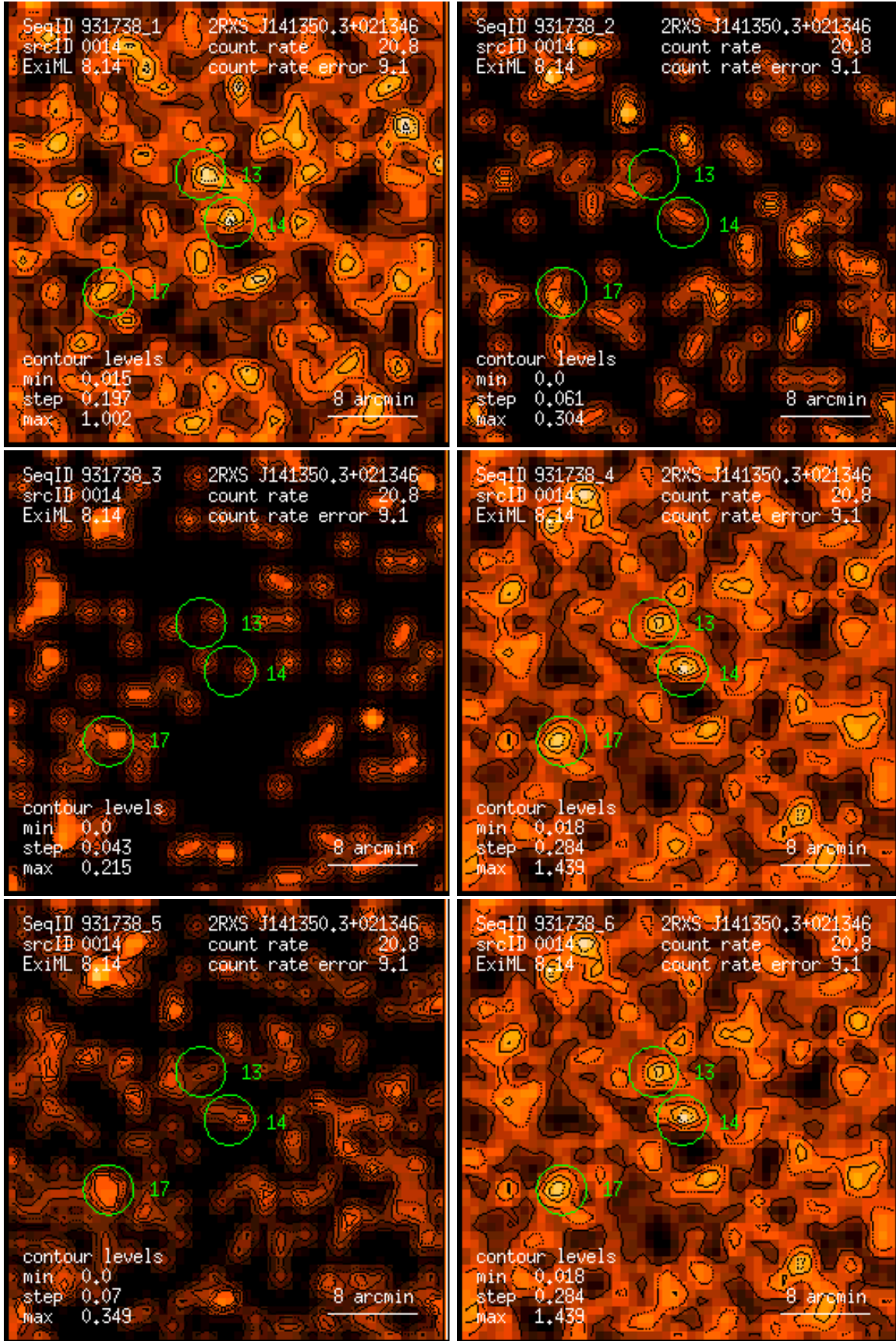
Figure 14: RASS 931738: detection 0014: band rate images, Gaussian filter: (1) PSPC channels 11 – 41, (2) 52 – 90, (3) 91 – 201, (4) 11 – 235, (5) 52 – 201, (6) 11 – 201. Broad band rates in counts/ks. Band rate contour levels in counts/ks/arcmin 2 .
