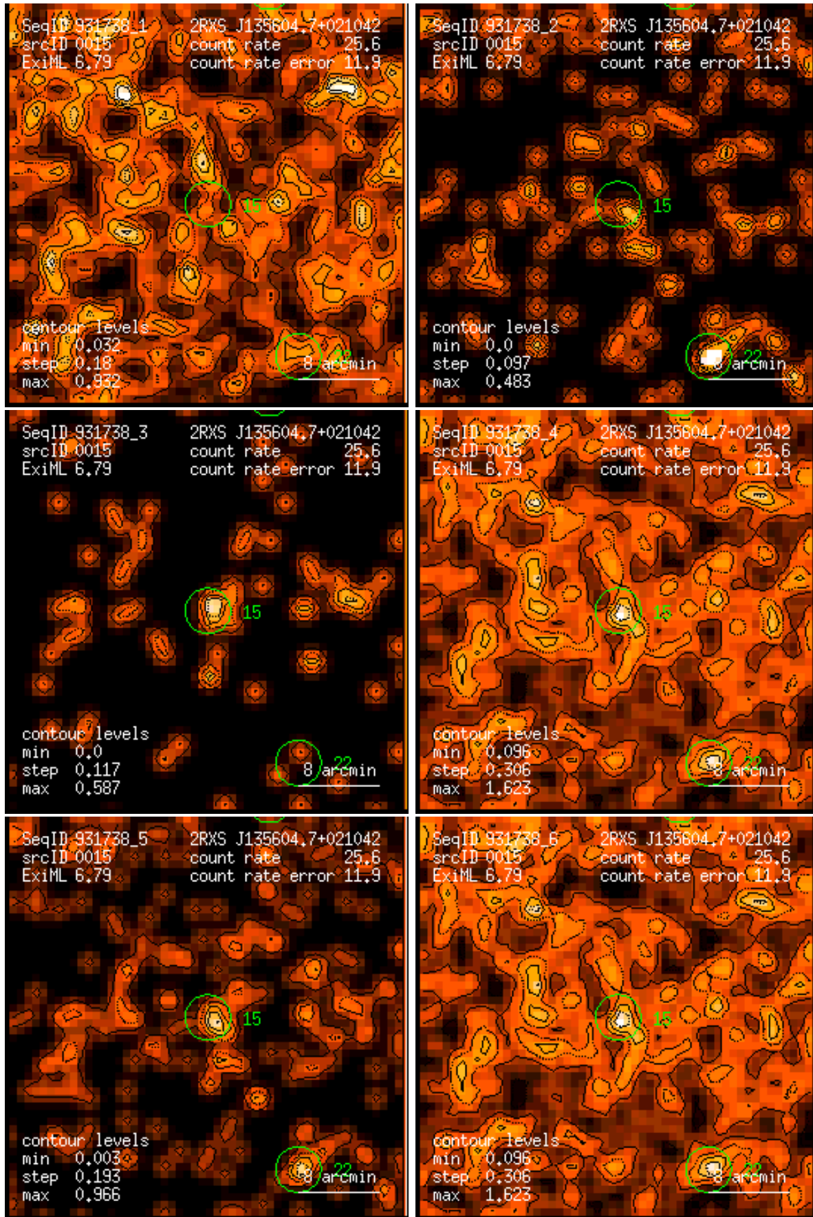
Figure 15: RASS 931738: detection 0015: band rate images, Gaussian filter: (1) PSPC channels 11 – 41, (2) 52 – 90, (3) 91 – 201, (4) 11 – 235, (5) 52 – 201, (6) 11 – 201. Broad band rates in counts/ks. Band rate contour levels in counts/ks/arcmin 2 .
