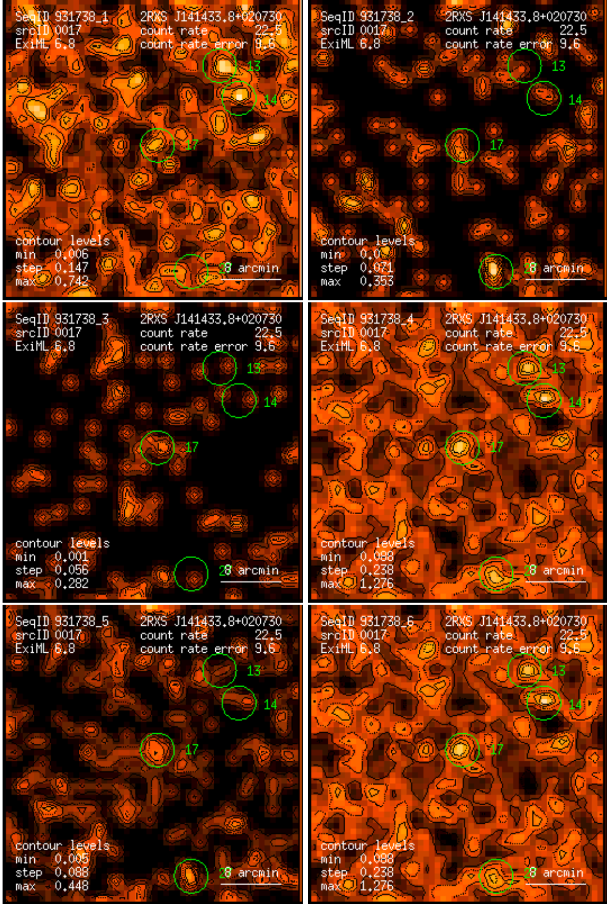
Figure 17: RASS 931738: detection 0017: band rate images, Gaussian filter: (1) PSPC channels 11 – 41, (2) 52 – 90, (3) 91 – 201, (4) 11 – 235, (5) 52 – 201, (6) 11 – 201. Broad band rates in counts/ks. Band rate contour levels in counts/ks/arcmin 2 .
