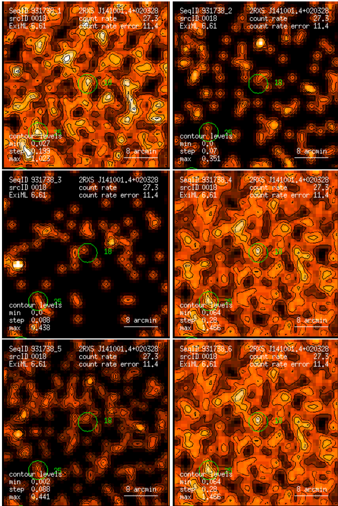
Figure 18: RASS 931738: detection 0018: band rate images, Gaussian filter: (1) PSPC channels 11 – 41, (2) 52 – 90, (3) 91 – 201, (4) 11 – 235, (5) 52 – 201, (6) 11 – 201. Broad band rates in counts/ks. Band rate contour levels in counts/ks/arcmin 2 .
