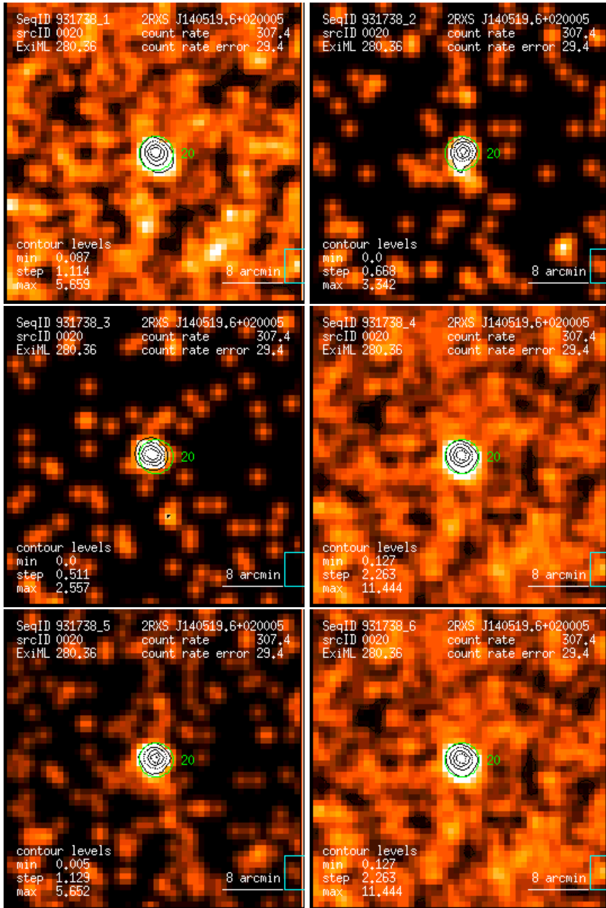
Figure 20: RASS 931738: detection 0020: band rate images, Gaussian filter: (1) PSPC channels 11 – 41, (2) 52 – 90, (3) 91 – 201, (4) 11 – 235, (5) 52 – 201, (6) 11 – 201. Broad band rates in counts/ks. Band rate contour levels in counts/ks/arcmin 2 .
