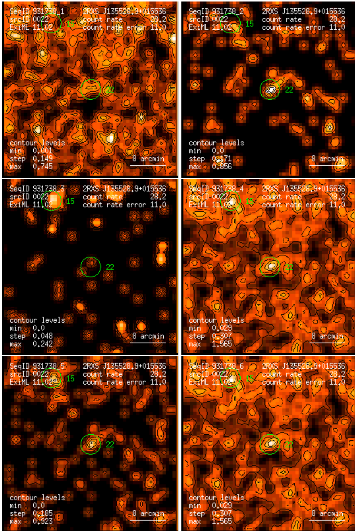
Figure 22: RASS 931738: detection 0022: band rate images, Gaussian filter: (1) PSPC channels 11 – 41, (2) 52 – 90, (3) 91 – 201, (4) 11 – 235, (5) 52 – 201, (6) 11 – 201. Broad band rates in counts/ks. Band rate contour levels in counts/ks/arcmin 2 .
