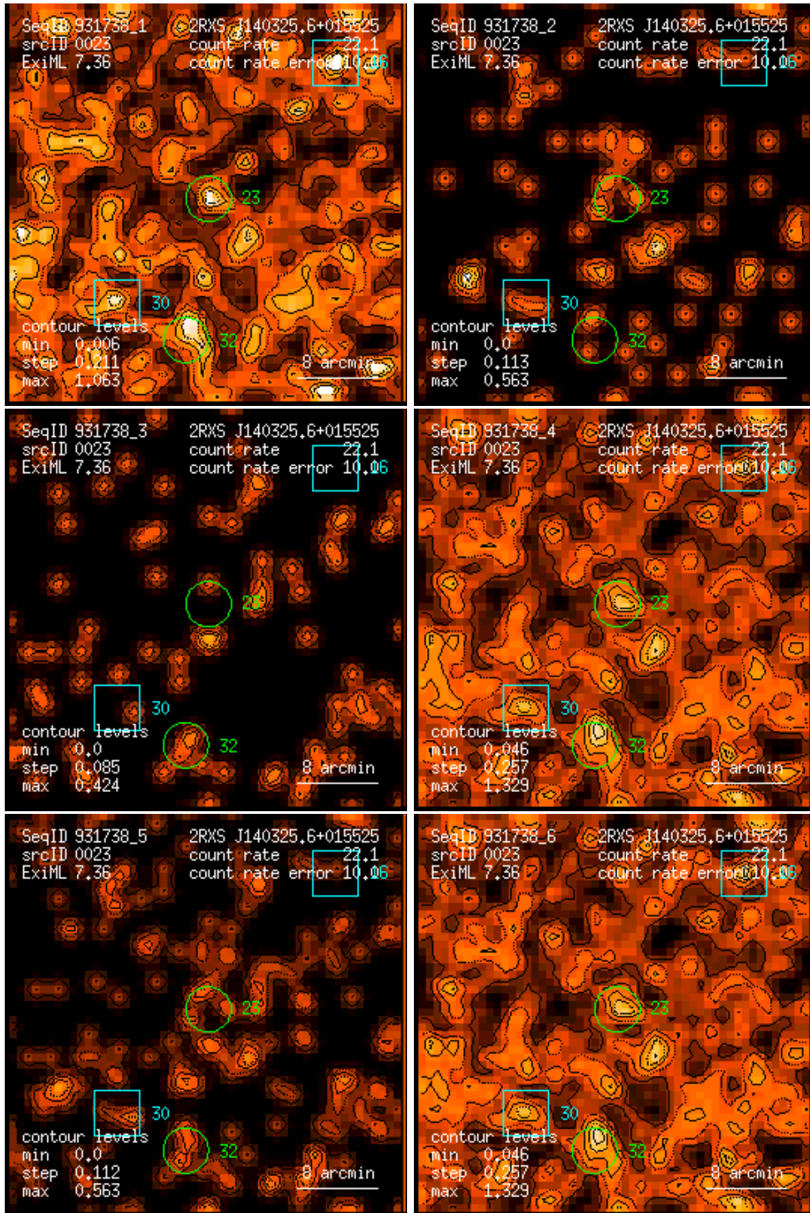
Figure 23: RASS 931738: detection 0023: band rate images, Gaussian filter: (1) PSPC channels 11 – 41, (2) 52 – 90, (3) 91 – 201, (4) 11 – 235, (5) 52 – 201, (6) 11 – 201. Broad band rates in counts/ks. Band rate contour levels in counts/ks/arcmin 2 .
