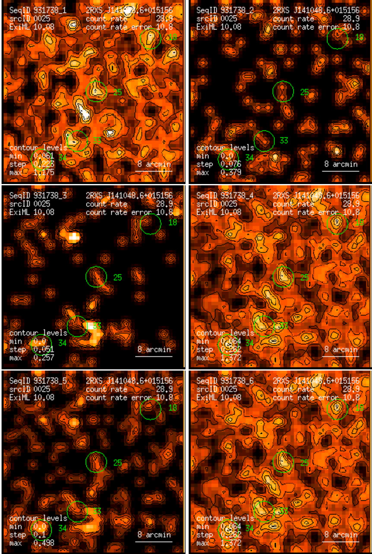
Figure 25: RASS 931738: detection 0025: band rate images, Gaussian filter: (1) PSPC channels 11 – 41, (2) 52 – 90, (3) 91 – 201, (4) 11 – 235, (5) 52 – 201, (6) 11 – 201. Broad band rates in counts/ks. Band rate contour levels in counts/ks/arcmin 2 .
