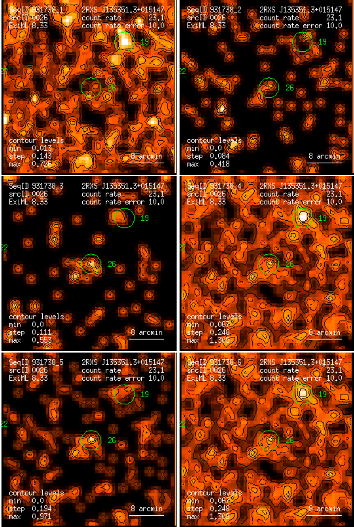
Figure 26: RASS 931738: detection 0026: band rate images, Gaussian filter: (1) PSPC channels 11 – 41, (2) 52 – 90, (3) 91 – 201, (4) 11 – 235, (5) 52 – 201, (6) 11 – 201. Broad band rates in counts/ks. Band rate contour levels in counts/ks/arcmin 2 .
