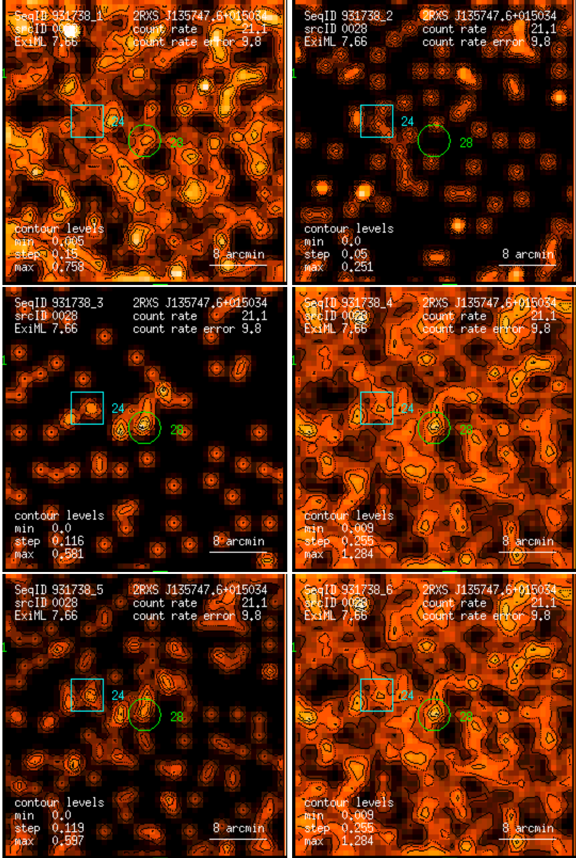
Figure 28: RASS 931738: detection 0028: band rate images, Gaussian filter: (1) PSPC channels 11 – 41, (2) 52 – 90, (3) 91 – 201, (4) 11 – 235, (5) 52 – 201, (6) 11 – 201. Broad band rates in counts/ks. Band rate contour levels in counts/ks/arcmin 2 .
