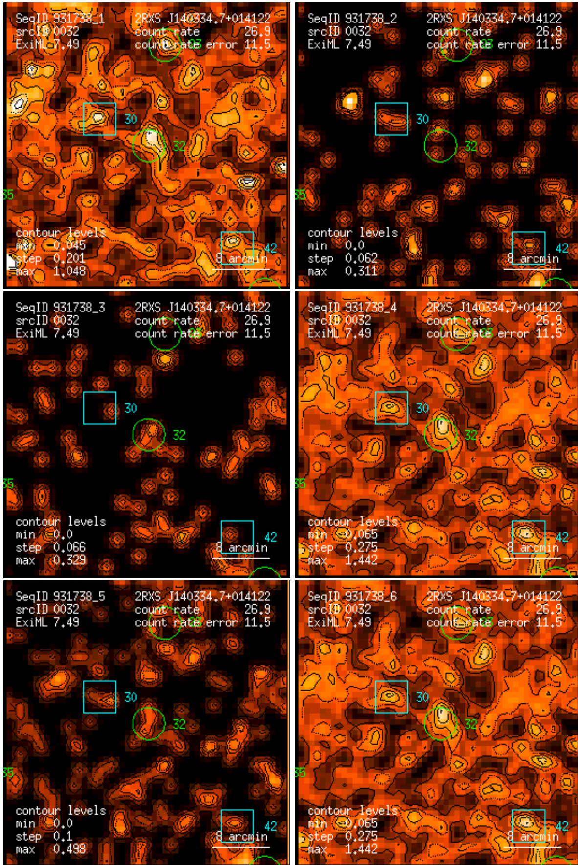
Figure 32: RASS 931738: detection 0032: band rate images, Gaussian filter: (1) PSPC channels 11 – 41, (2) 52 – 90, (3) 91 – 201, (4) 11 – 235, (5) 52 – 201, (6) 11 – 201. Broad band rates in counts/ks. Band rate contour levels in counts/ks/arcmin 2 .
