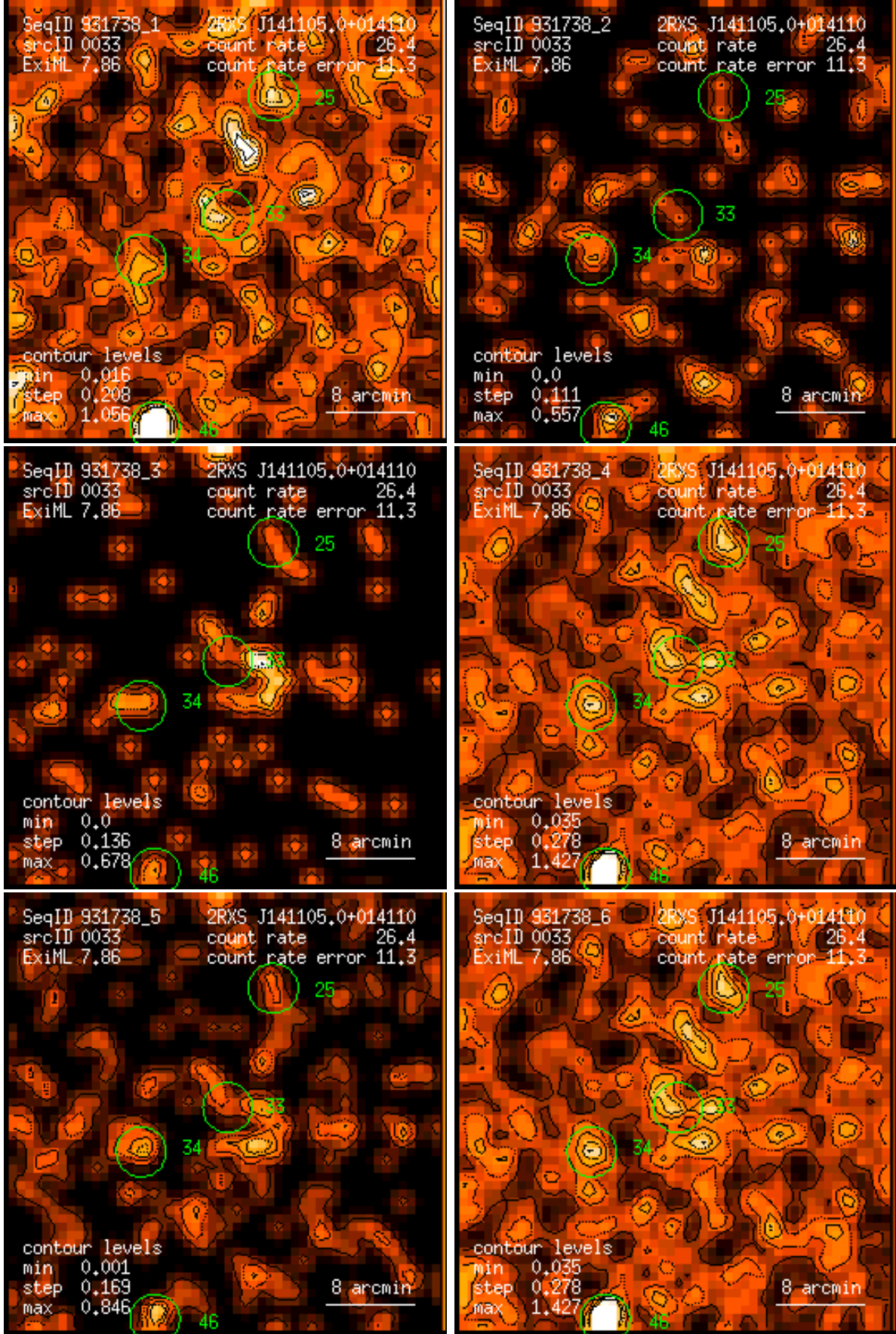
Figure 33: RASS 931738: detection 0033: band rate images, Gaussian filter: (1) PSPC channels 11 – 41, (2) 52 – 90, (3) 91 – 201, (4) 11 – 235, (5) 52 – 201, (6) 11 – 201. Broad band rates in counts/ks. Band rate contour levels in counts/ks/arcmin 2 .
