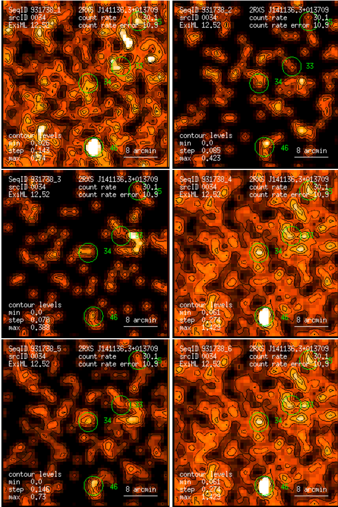
Figure 34: RASS 931738: detection 0034: band rate images, Gaussian filter: (1) PSPC channels 11 – 41, (2) 52 – 90, (3) 91 – 201, (4) 11 – 235, (5) 52 – 201, (6) 11 – 201. Broad band rates in counts/ks. Band rate contour levels in counts/ks/arcmin 2 .
