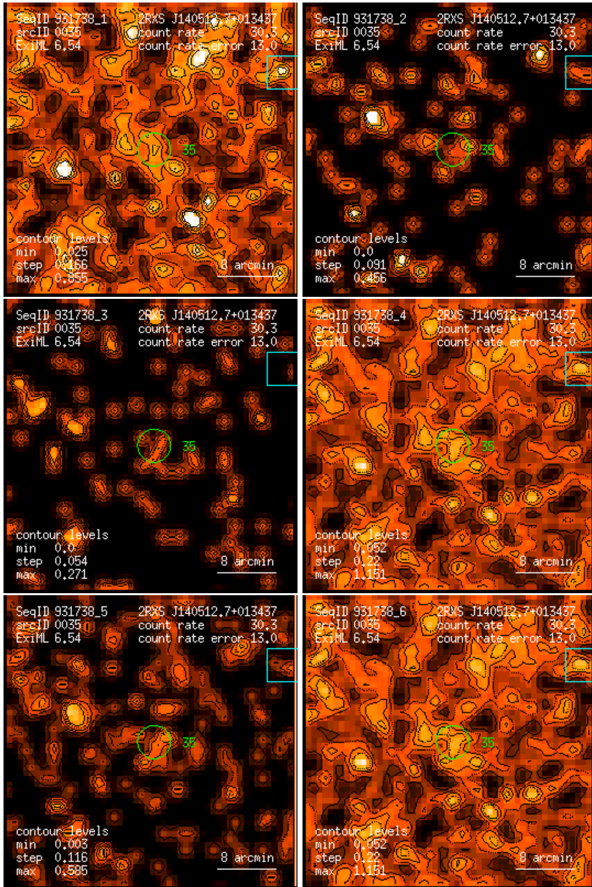
Figure 35: RASS 931738: detection 0035: band rate images, Gaussian filter: (1) PSPC channels 11 – 41, (2) 52 – 90, (3) 91 – 201, (4) 11 – 235, (5) 52 – 201, (6) 11 – 201. Broad band rates in counts/ks. Band rate contour levels in counts/ks/arcmin 2 .
