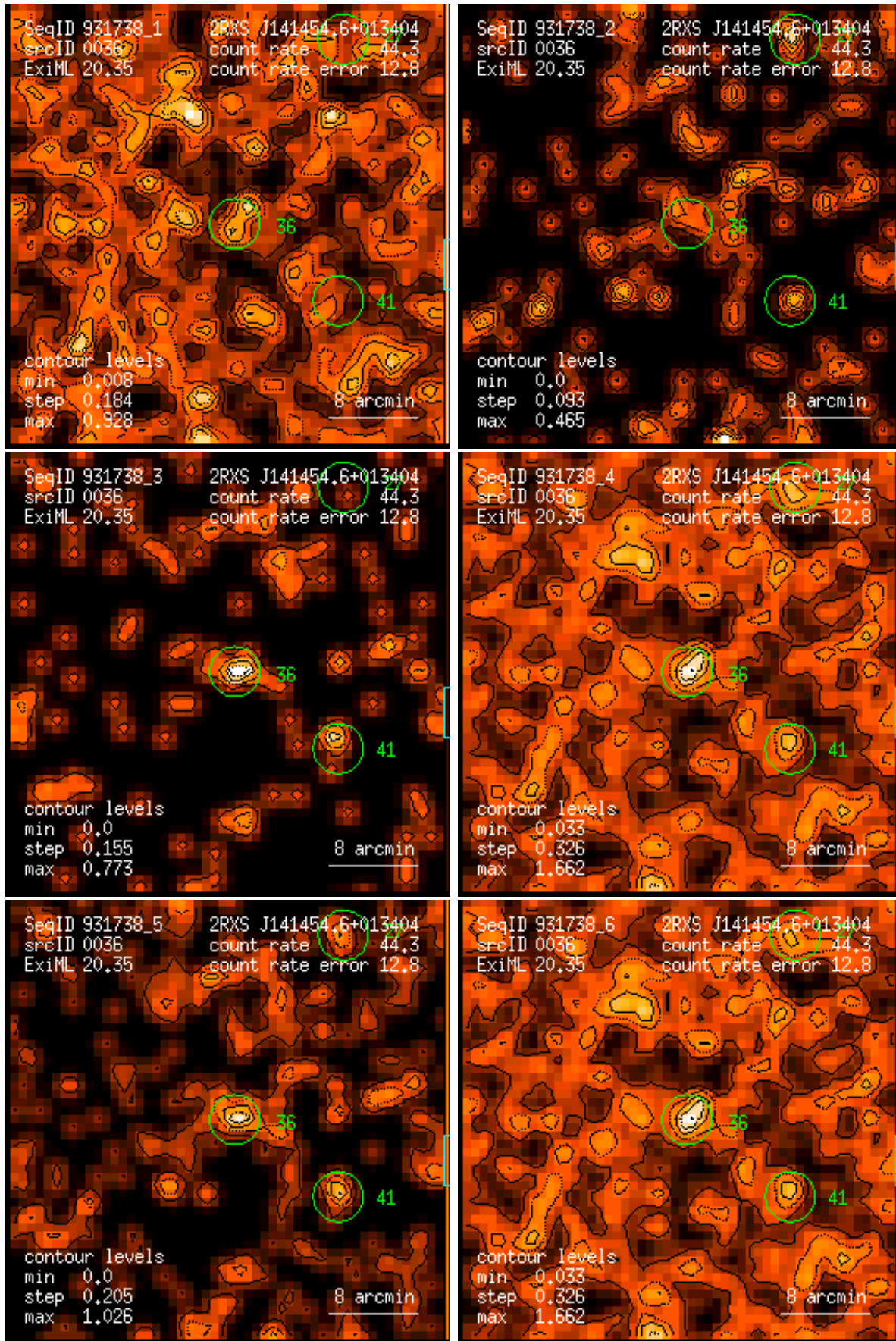
Figure 36: RASS 931738: detection 0036: band rate images, Gaussian filter: (1) PSPC channels 11 – 41, (2) 52 – 90, (3) 91 – 201, (4) 11 – 235, (5) 52 – 201, (6) 11 – 201. Broad band rates in counts/ks. Band rate contour levels in counts/ks/arcmin 2 .
