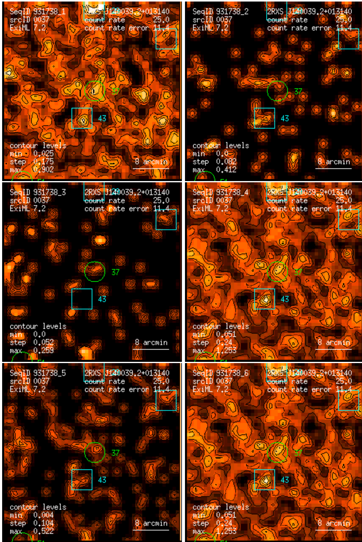
Figure 37: RASS 931738: detection 0037: band rate images, Gaussian filter: (1) PSPC channels 11 – 41, (2) 52 – 90, (3) 91 – 201, (4) 11 – 235, (5) 52 – 201, (6) 11 – 201. Broad band rates in counts/ks. Band rate contour levels in counts/ks/arcmin 2 .
