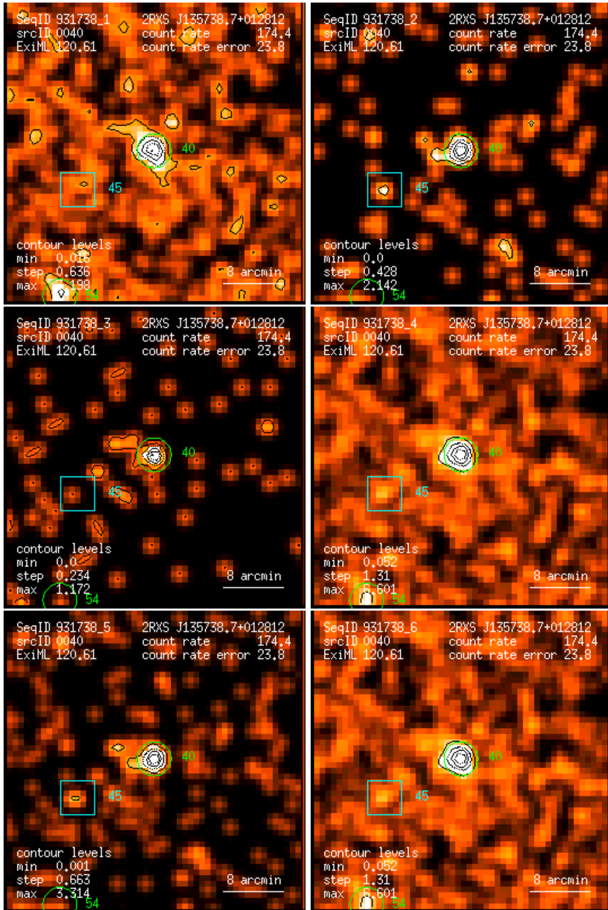
Figure 40: RASS 931738: detection 0040: band rate images, Gaussian filter: (1) PSPC channels 11 – 41, (2) 52 – 90, (3) 91 – 201, (4) 11 – 235, (5) 52 – 201, (6) 11 – 201. Broad band rates in counts/ks. Band rate contour levels in counts/ks/arcmin 2 .
