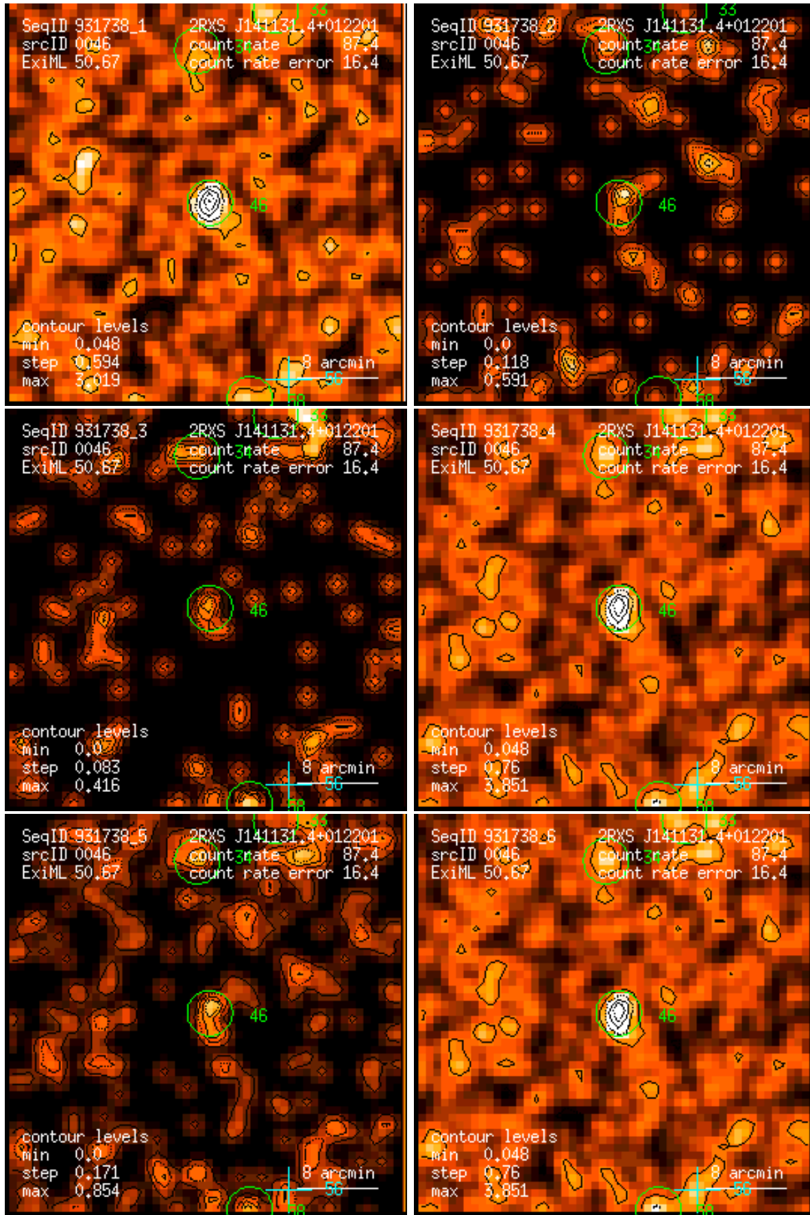
Figure 46: RASS 931738: detection 0046: band rate images, Gaussian filter: (1) PSPC channels 11 – 41, (2) 52 – 90, (3) 91 – 201, (4) 11 – 235, (5) 52 – 201, (6) 11 – 201. Broad band rates in counts/ks. Band rate contour levels in counts/ks/arcmin 2 .
