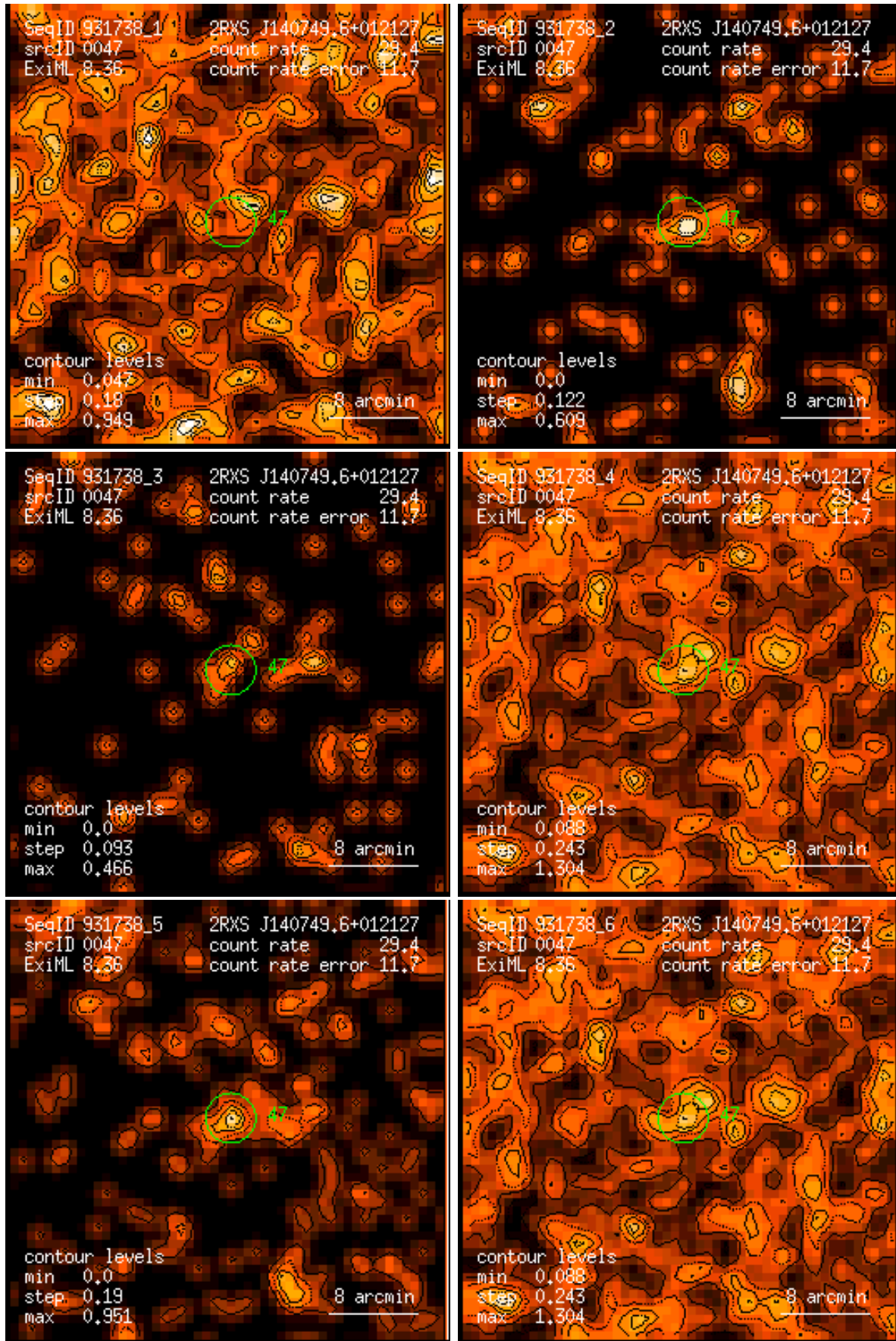
Figure 47: RASS 931738: detection 0047: band rate images, Gaussian filter: (1) PSPC channels 11 – 41, (2) 52 – 90, (3) 91 – 201, (4) 11 – 235, (5) 52 – 201, (6) 11 – 201. Broad band rates in counts/ks. Band rate contour levels in counts/ks/arcmin 2 .
