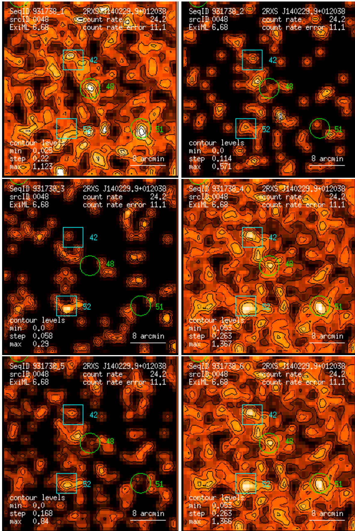
Figure 48: RASS 931738: detection 0048: band rate images, Gaussian filter: (1) PSPC channels 11 – 41, (2) 52 – 90, (3) 91 – 201, (4) 11 – 235, (5) 52 – 201, (6) 11 – 201. Broad band rates in counts/ks. Band rate contour levels in counts/ks/arcmin 2 .
