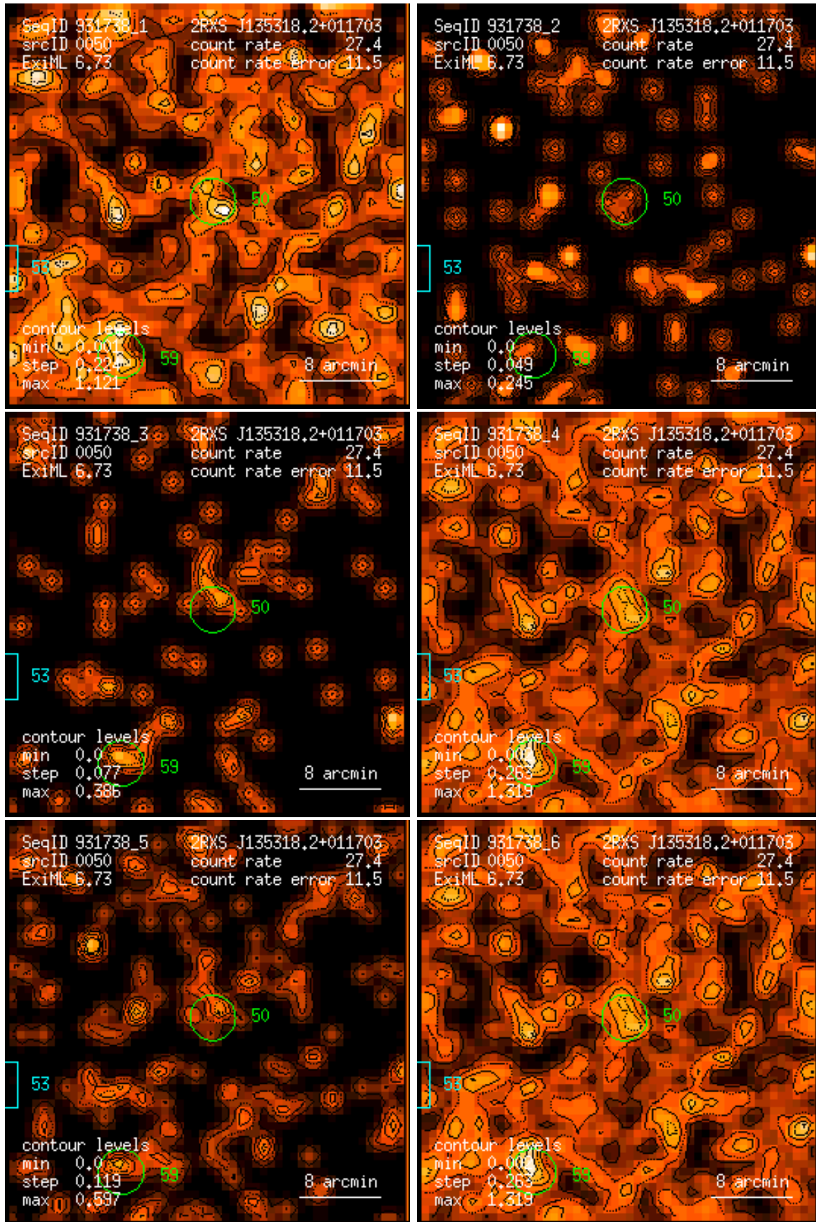
Figure 50: RASS 931738: detection 0050: band rate images, Gaussian filter: (1) PSPC channels 11 – 41, (2) 52 – 90, (3) 91 – 201, (4) 11 – 235, (5) 52 – 201, (6) 11 – 201. Broad band rates in counts/ks. Band rate contour levels in counts/ks/arcmin 2 .
