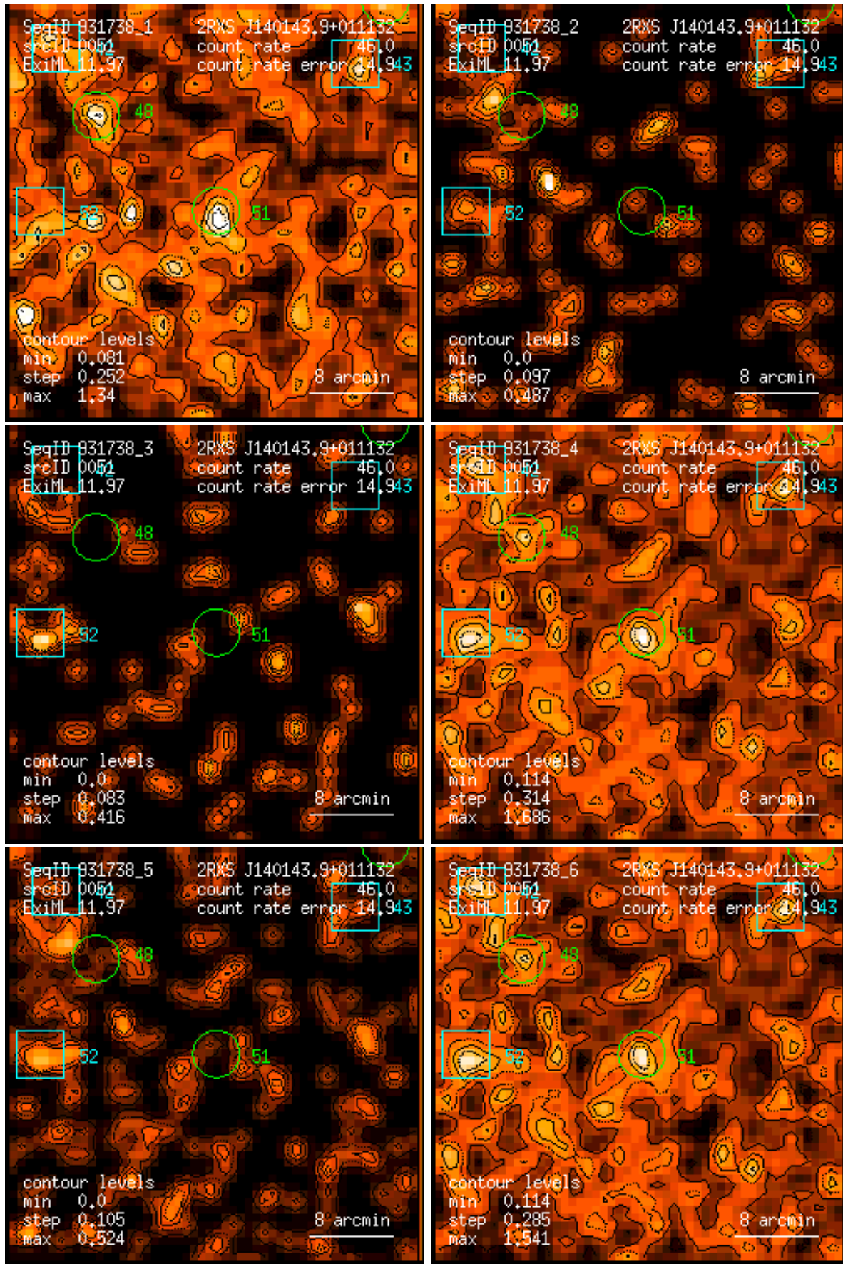
Figure 51: RASS 931738: detection 0051: band rate images, Gaussian filter: (1) PSPC channels 11 – 41, (2) 52 – 90, (3) 91 – 201, (4) 11 – 235, (5) 52 – 201, (6) 11 – 201. Broad band rates in counts/ks. Band rate contour levels in counts/ks/arcmin 2 .
