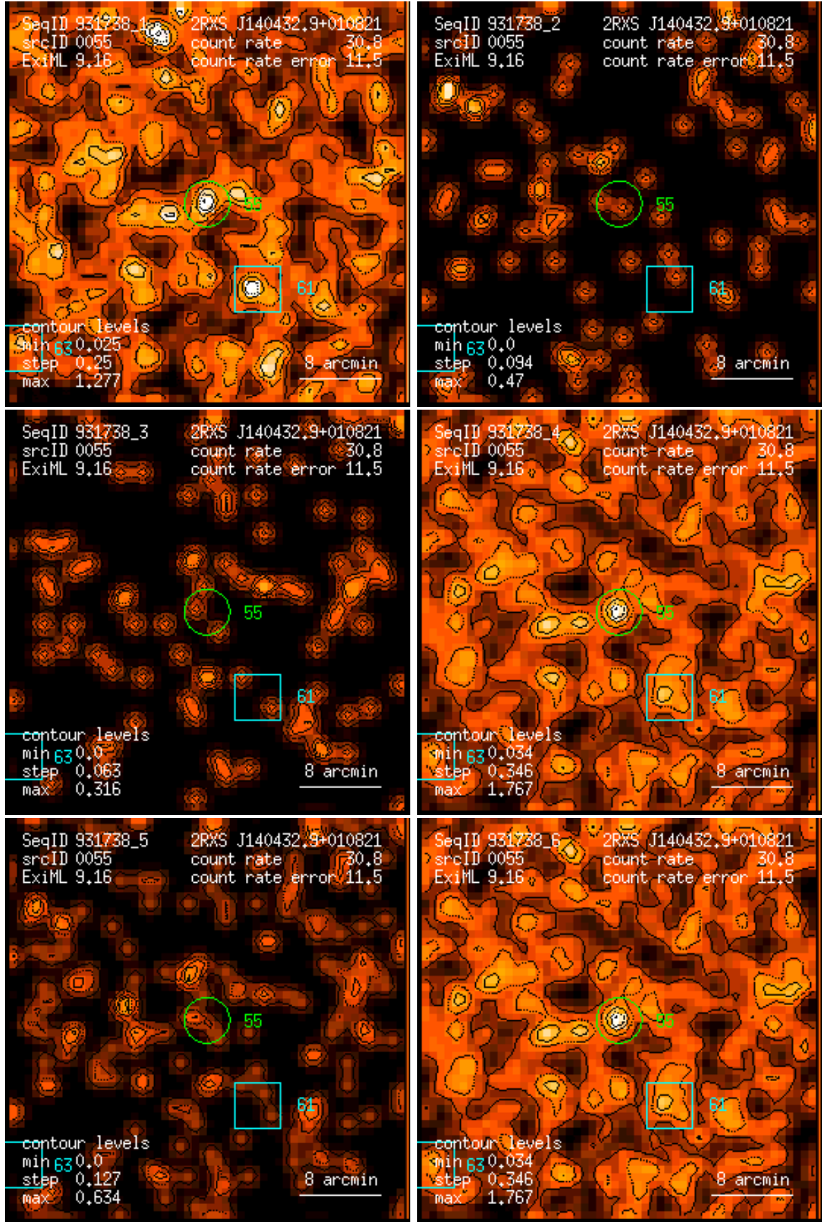
Figure 55: RASS 931738: detection 0055: band rate images, Gaussian filter: (1) PSPC channels 11 – 41, (2) 52 – 90, (3) 91 – 201, (4) 11 – 235, (5) 52 – 201, (6) 11 – 201. Broad band rates in counts/ks. Band rate contour levels in counts/ks/arcmin 2 .
