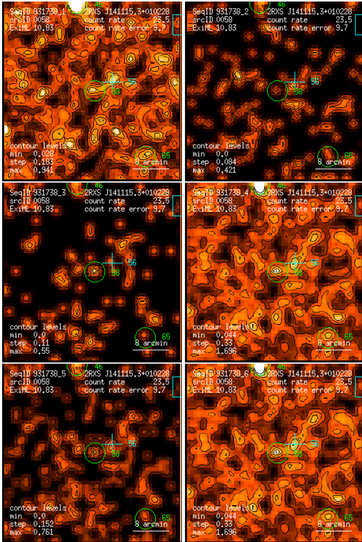
Figure 58: RASS 931738: detection 0058: band rate images, Gaussian filter: (1) PSPC channels 11 – 41, (2) 52 – 90, (3) 91 – 201, (4) 11 – 235, (5) 52 – 201, (6) 11 – 201. Broad band rates in counts/ks. Band rate contour levels in counts/ks/arcmin 2 .
