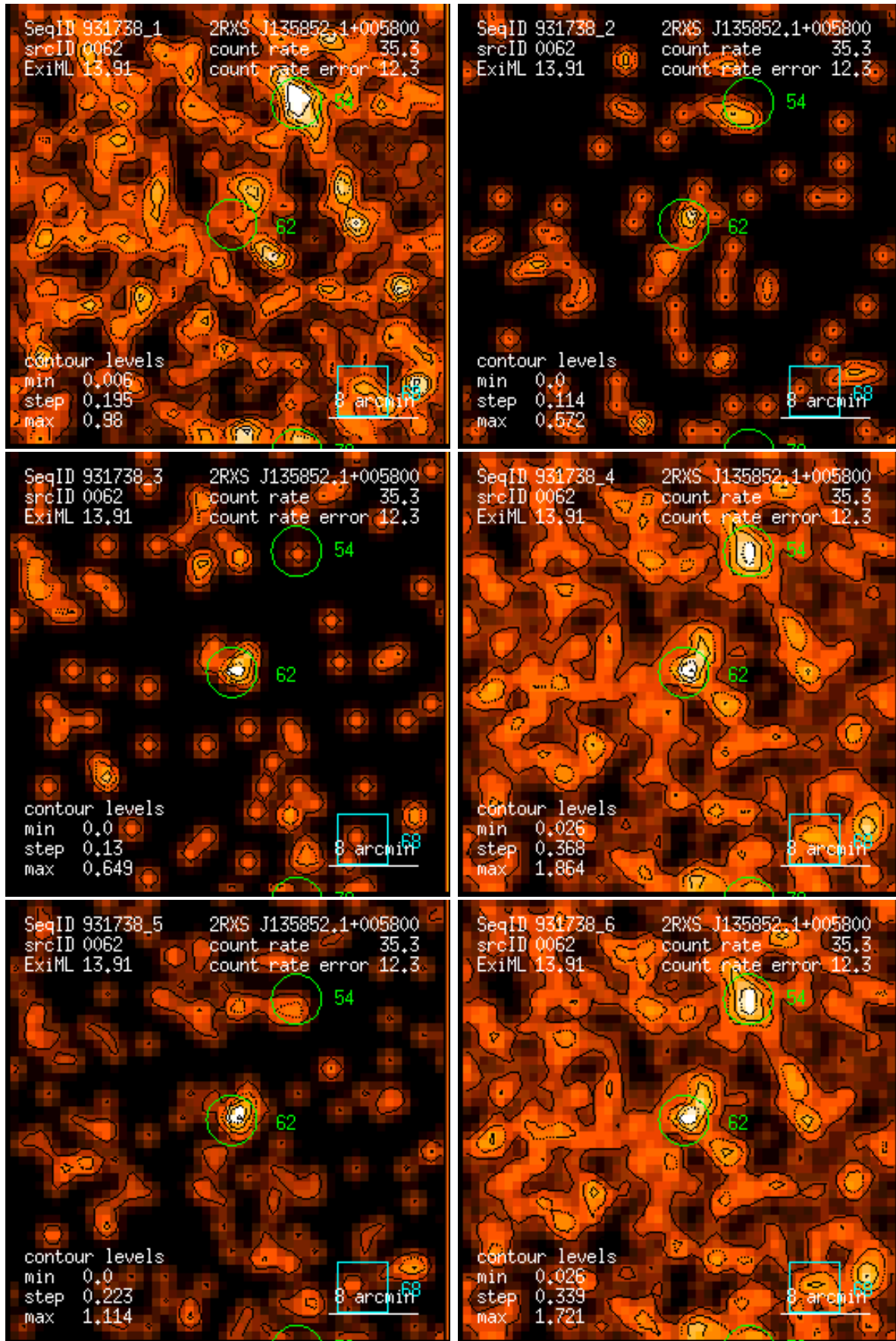
Figure 62: RASS 931738: detection 0062: band rate images, Gaussian filter: (1) PSPC channels 11 – 41, (2) 52 – 90, (3) 91 – 201, (4) 11 – 235, (5) 52 – 201, (6) 11 – 201. Broad band rates in counts/ks. Band rate contour levels in counts/ks/arcmin 2 .
