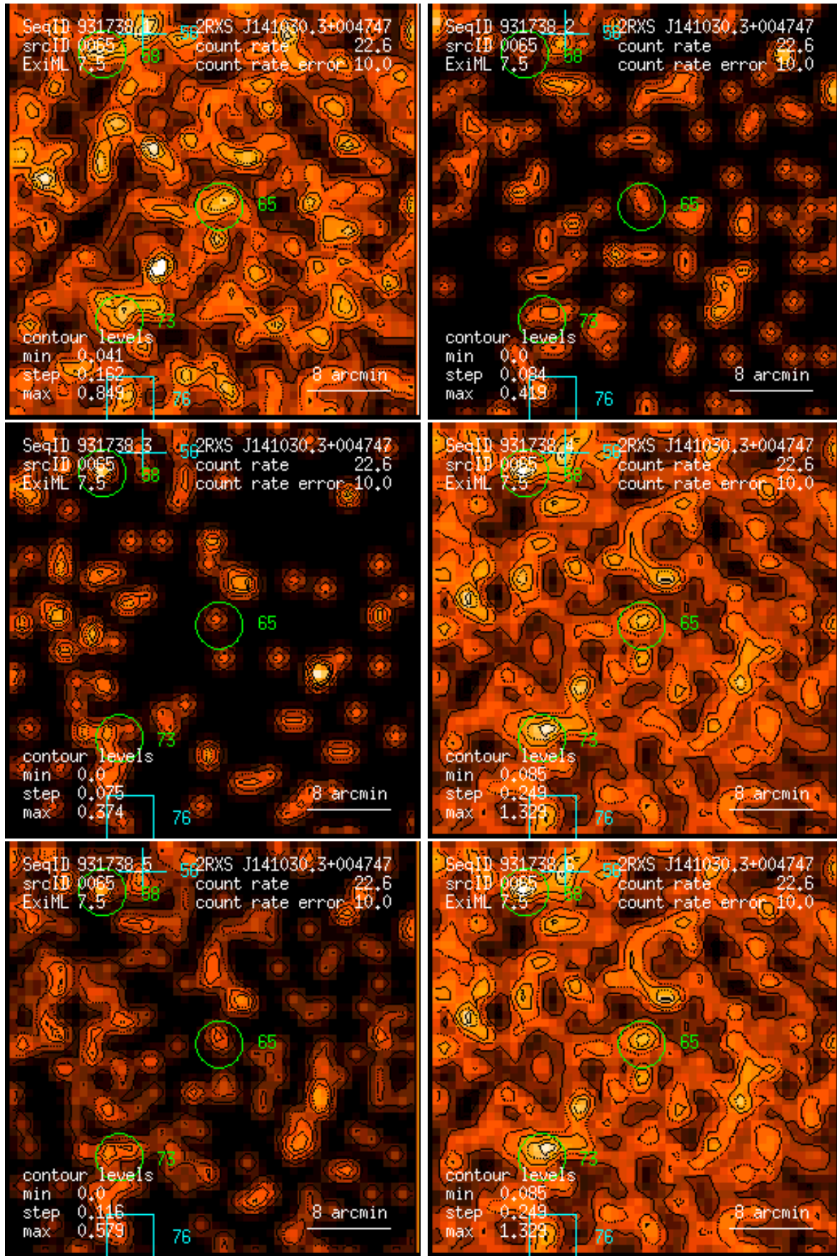
Figure 65: RASS 931738: detection 0065: band rate images, Gaussian filter: (1) PSPC channels 11 – 41, (2) 52 – 90, (3) 91 – 201, (4) 11 – 235, (5) 52 – 201, (6) 11 – 201. Broad band rates in counts/ks. Band rate contour levels in counts/ks/arcmin 2 .
