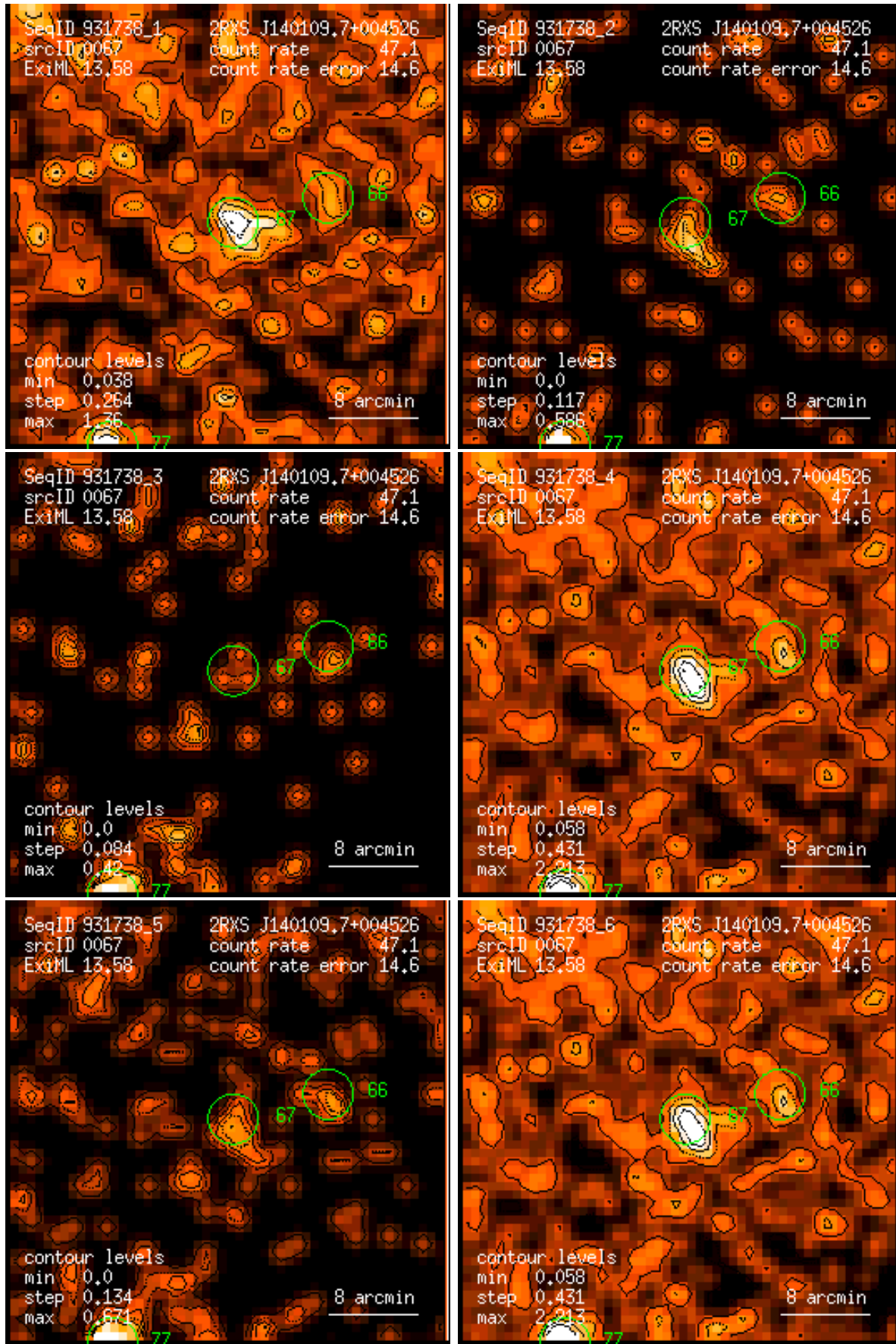
Figure 67: RASS 931738: detection 0067: band rate images, Gaussian filter: (1) PSPC channels 11 – 41, (2) 52 – 90, (3) 91 – 201, (4) 11 – 235, (5) 52 – 201, (6) 11 – 201. Broad band rates in counts/ks. Band rate contour levels in counts/ks/arcmin 2 .
