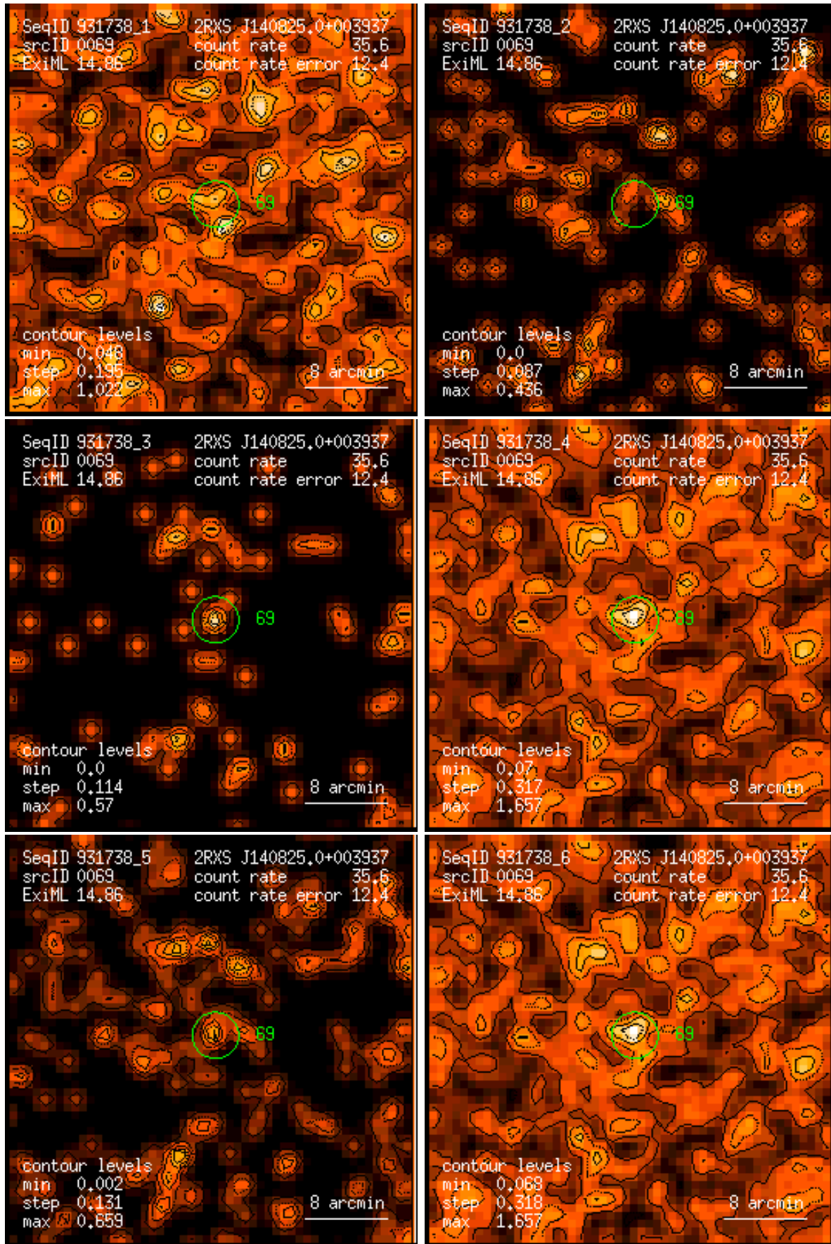
Figure 69: RASS 931738: detection 0069: band rate images, Gaussian filter: (1) PSPC channels 11 – 41, (2) 52 – 90, (3) 91 – 201, (4) 11 – 235, (5) 52 – 201, (6) 11 – 201. Broad band rates in counts/ks. Band rate contour levels in counts/ks/arcmin 2 .
