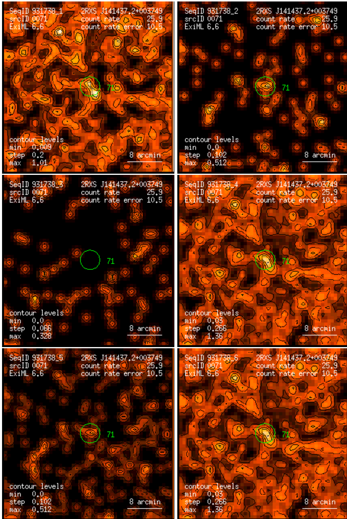
Figure 71: RASS 931738: detection 0071: band rate images, Gaussian filter: (1) PSPC channels 11 – 41, (2) 52 – 90, (3) 91 – 201, (4) 11 – 235, (5) 52 – 201, (6) 11 – 201. Broad band rates in counts/ks. Band rate contour levels in counts/ks/arcmin 2 .
