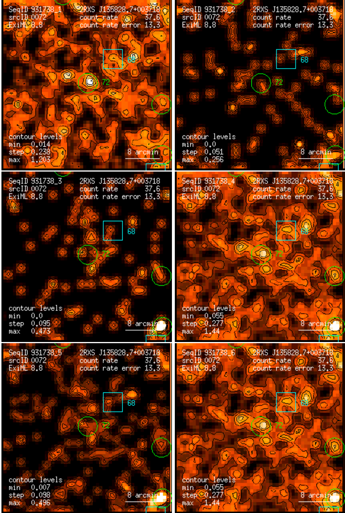
Figure 72: RASS 931738: detection 0072: band rate images, Gaussian filter: (1) PSPC channels 11 – 41, (2) 52 – 90, (3) 91 – 201, (4) 11 – 235, (5) 52 – 201, (6) 11 – 201. Broad band rates in counts/ks. Band rate contour levels in counts/ks/arcmin 2 .
