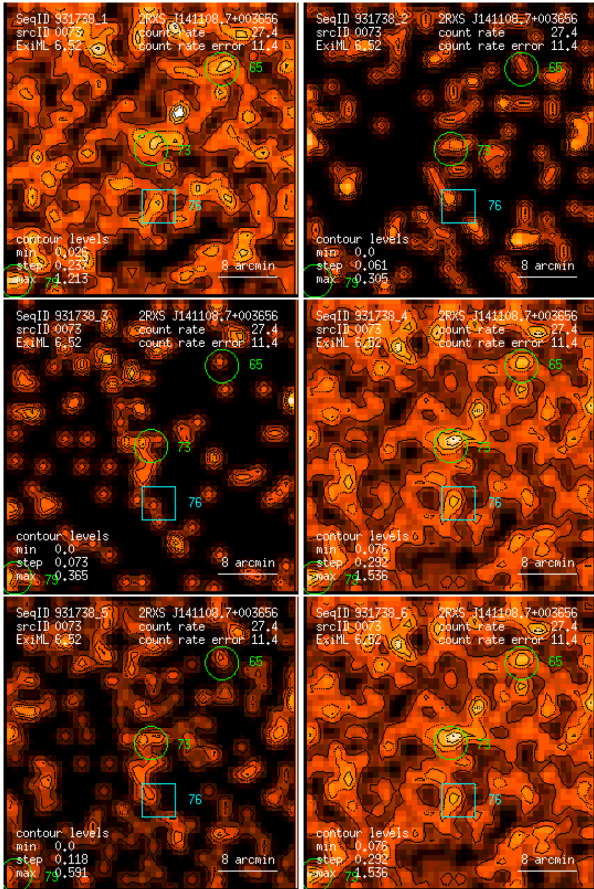
Figure 73: RASS 931738: detection 0073: band rate images, Gaussian filter: (1) PSPC channels 11 – 41, (2) 52 – 90, (3) 91 – 201, (4) 11 – 235, (5) 52 – 201, (6) 11 – 201. Broad band rates in counts/ks. Band rate contour levels in counts/ks/arcmin 2 .
