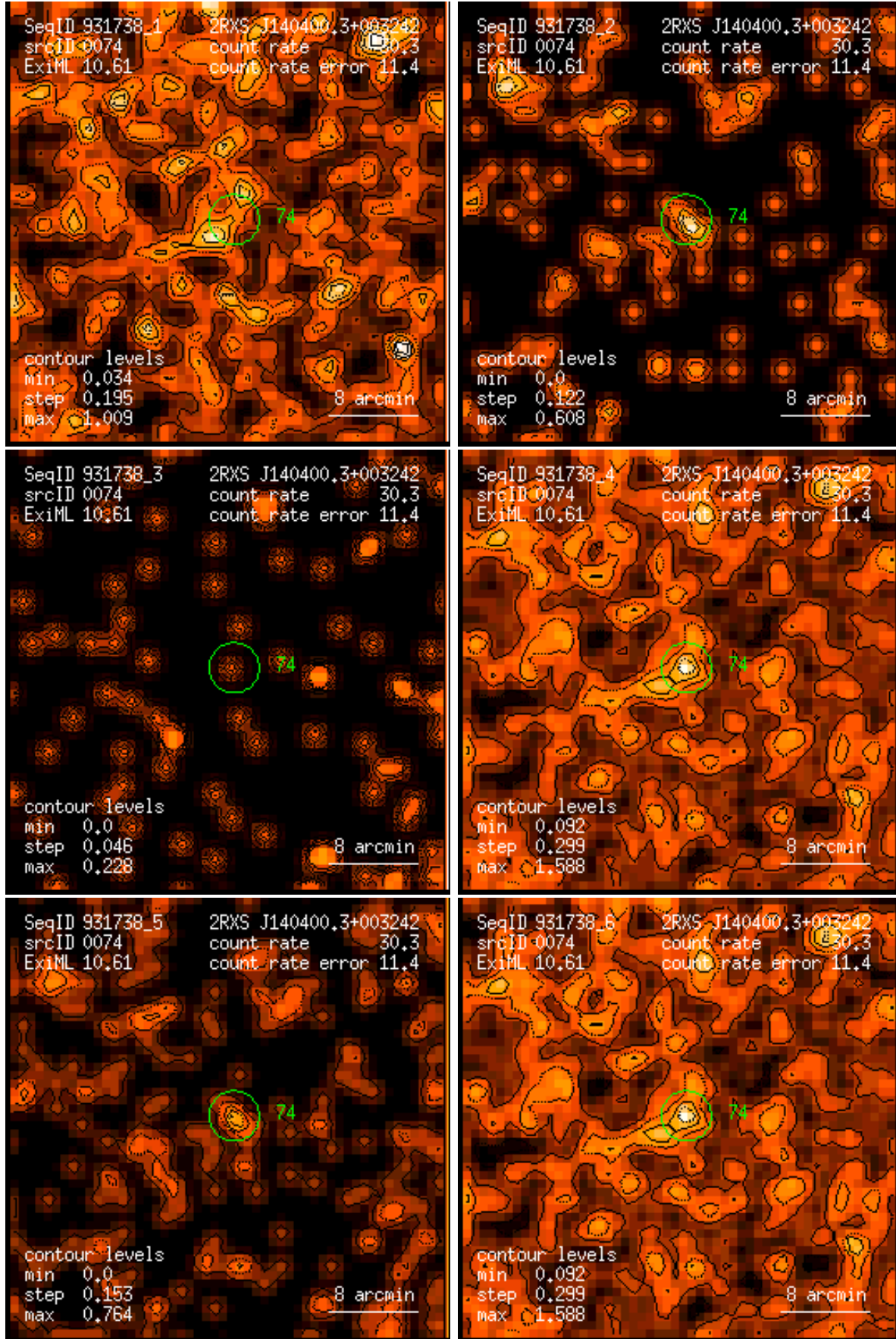
Figure 74: RASS 931738: detection 0074: band rate images, Gaussian filter: (1) PSPC channels 11 – 41, (2) 52 – 90, (3) 91 – 201, (4) 11 – 235, (5) 52 – 201, (6) 11 – 201. Broad band rates in counts/ks. Band rate contour levels in counts/ks/arcmin 2 .
