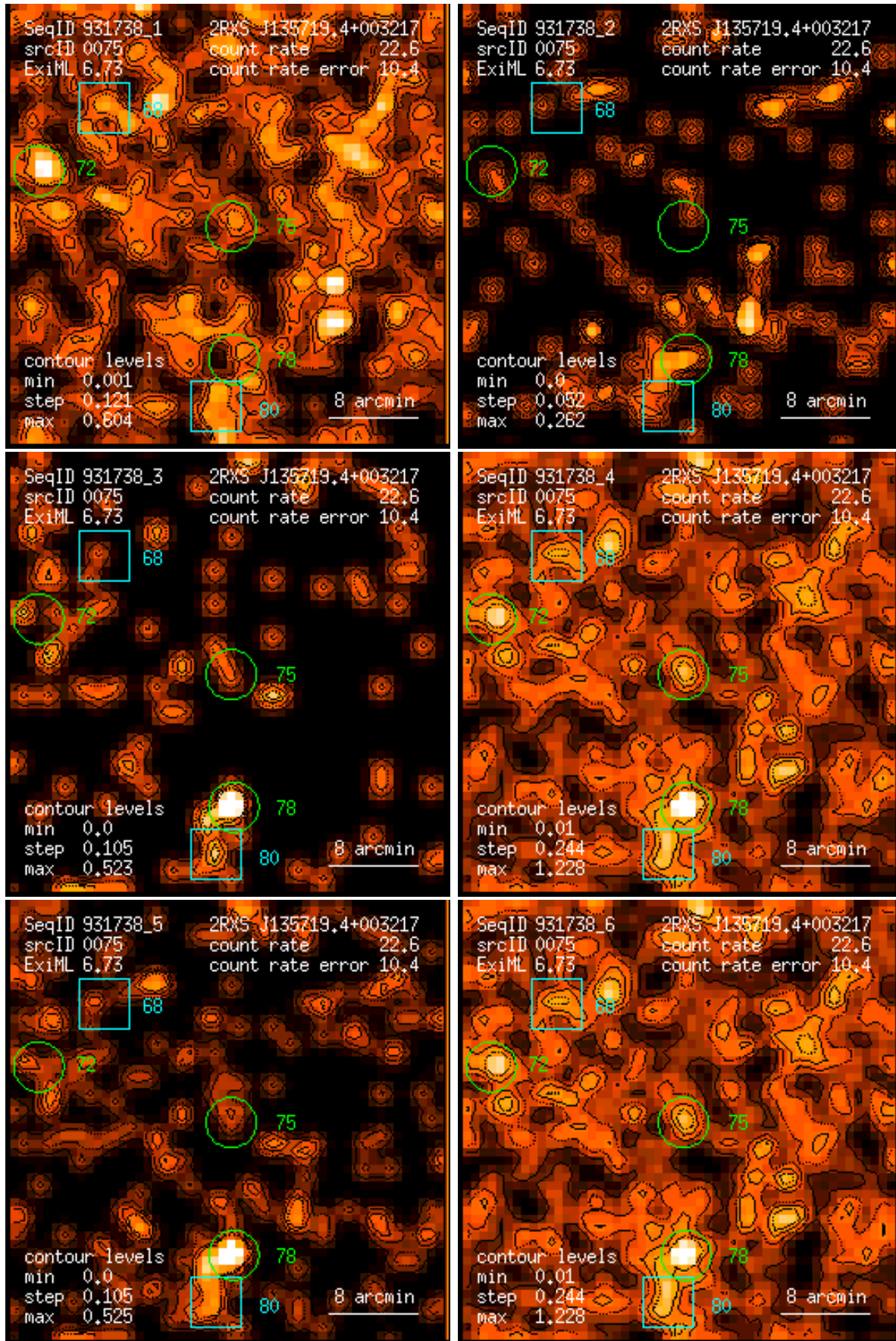
Figure 75: RASS 931738: detection 0075: band rate images, Gaussian filter: (1) PSPC channels 11 – 41, (2) 52 – 90, (3) 91 – 201, (4) 11 – 235, (5) 52 – 201, (6) 11 – 201. Broad band rates in counts/ks. Band rate contour levels in counts/ks/arcmin 2 .
