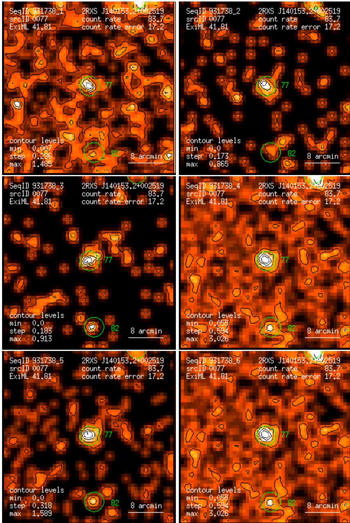
Figure 77: RASS 931738: detection 0077: band rate images, Gaussian filter: (1) PSPC channels 11 – 41, (2) 52 – 90, (3) 91 – 201, (4) 11 – 235, (5) 52 – 201, (6) 11 – 201. Broad band rates in counts/ks. Band rate contour levels in counts/ks/arcmin 2 .
