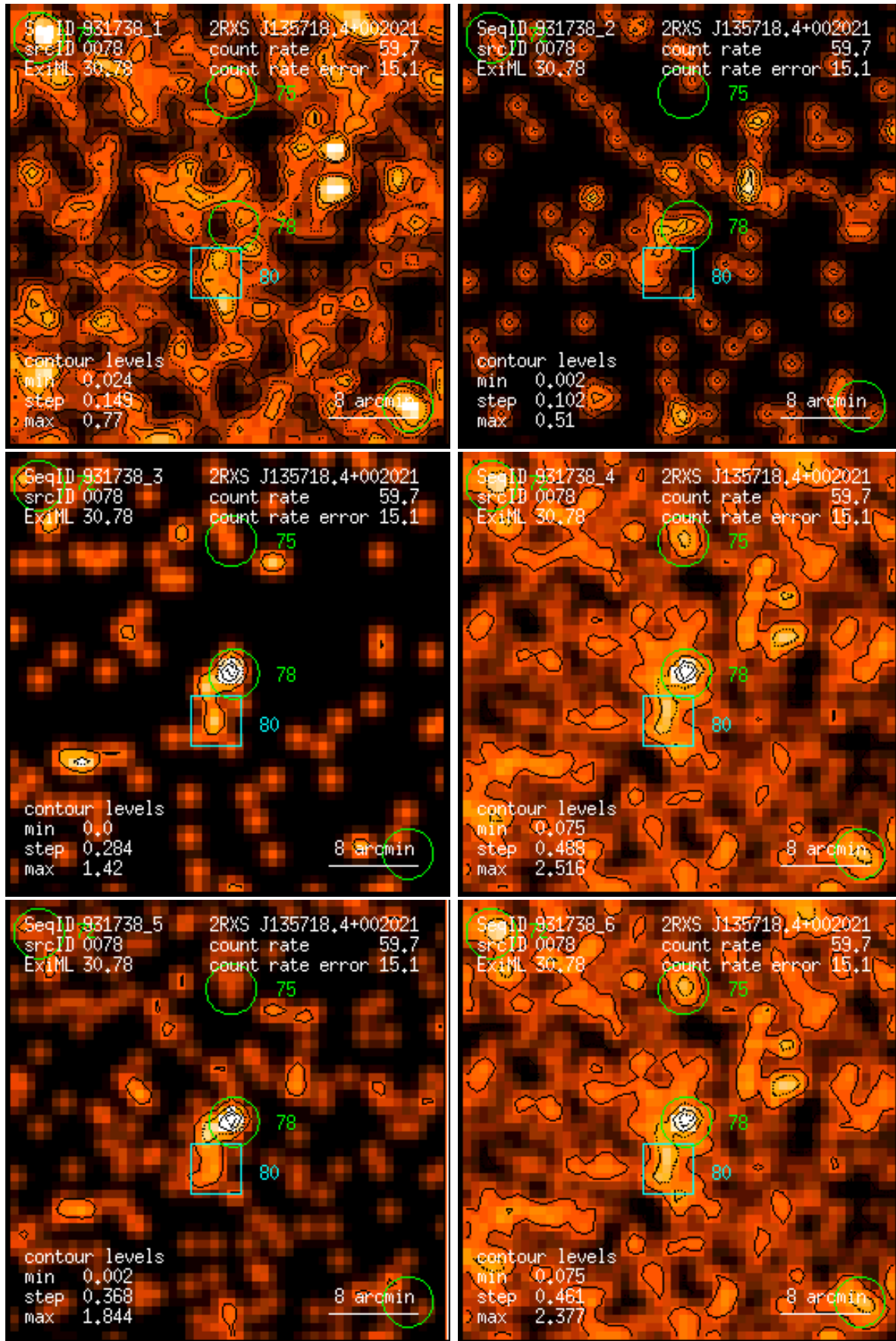
Figure 78: RASS 931738: detection 0078: band rate images, Gaussian filter: (1) PSPC channels 11 – 41, (2) 52 – 90, (3) 91 – 201, (4) 11 – 235, (5) 52 – 201, (6) 11 – 201. Broad band rates in counts/ks. Band rate contour levels in counts/ks/arcmin 2 .
