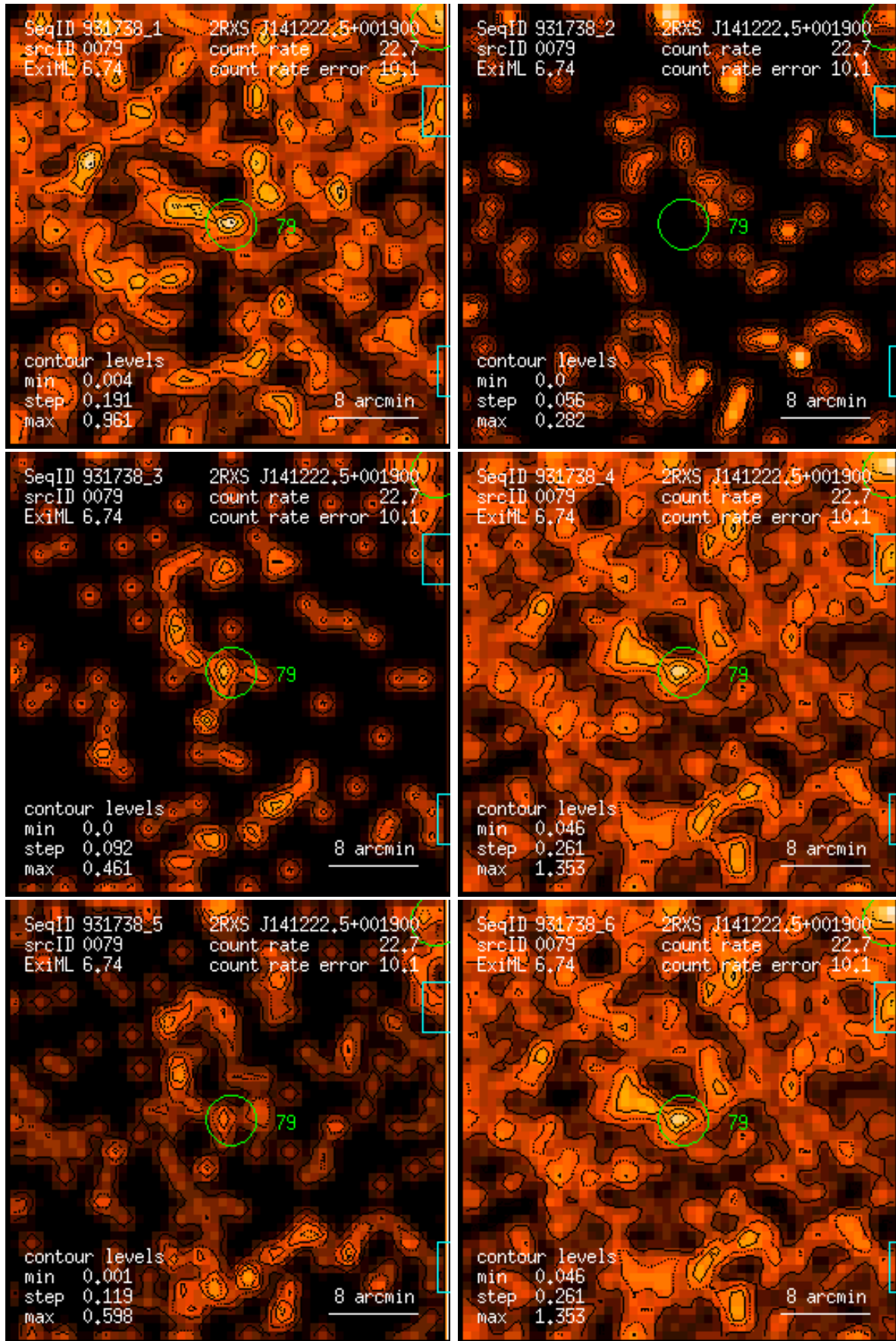
Figure 79: RASS 931738: detection 0079: band rate images, Gaussian filter: (1) PSPC channels 11 – 41, (2) 52 – 90, (3) 91 – 201, (4) 11 – 235, (5) 52 – 201, (6) 11 – 201. Broad band rates in counts/ks. Band rate contour levels in counts/ks/arcmin 2 .
