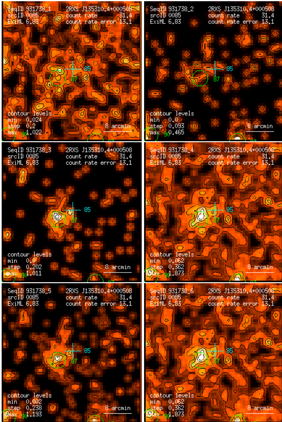
Figure 85: RASS 931738: detection 0085: band rate images, Gaussian filter: (1) PSPC channels 11 – 41, (2) 52 – 90, (3) 91 – 201, (4) 11 – 235, (5) 52 – 201, (6) 11 – 201. Broad band rates in counts/ks. Band rate contour levels in counts/ks/arcmin 2 .
