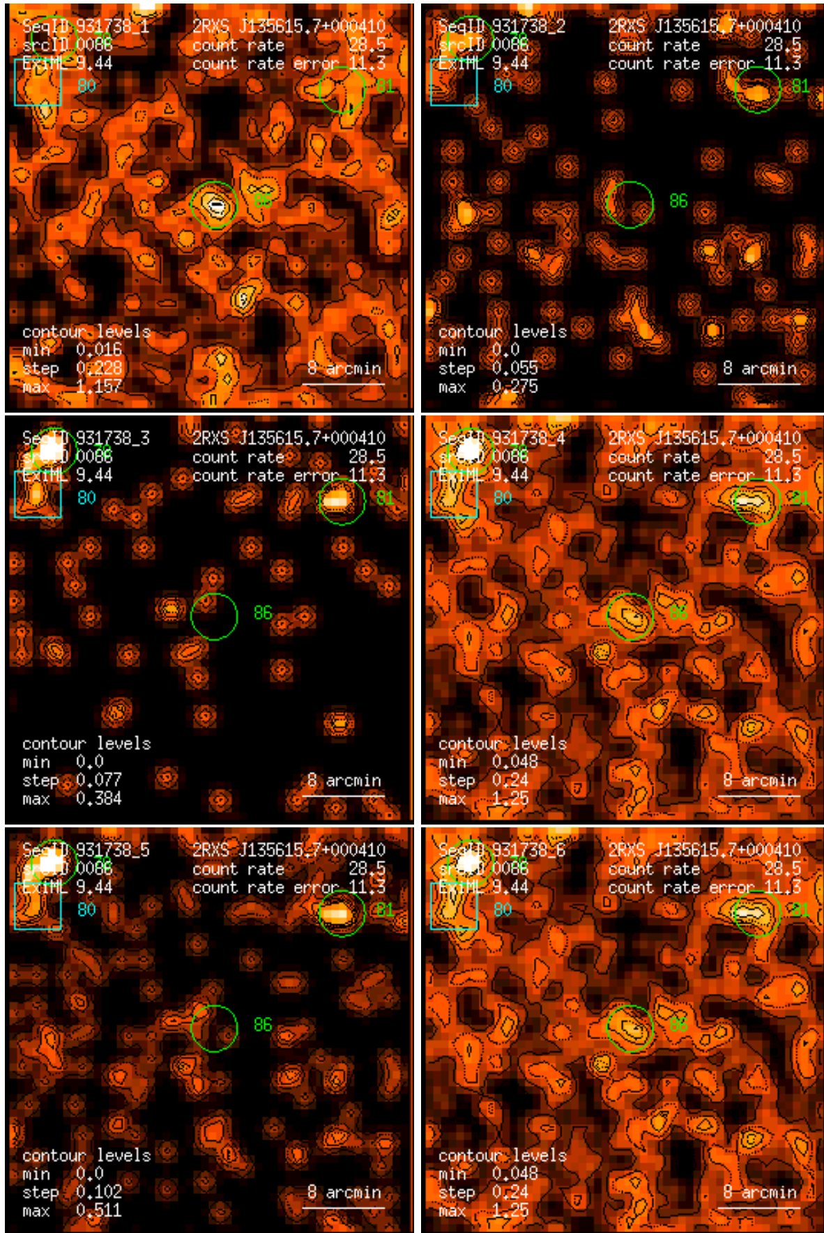
Figure 86: RASS 931738: detection 0086: band rate images, Gaussian filter: (1) PSPC channels 11 – 41, (2) 52 – 90, (3) 91 – 201, (4) 11 – 235, (5) 52 – 201, (6) 11 – 201. Broad band rates in counts/ks. Band rate contour levels in counts/ks/arcmin 2 .
