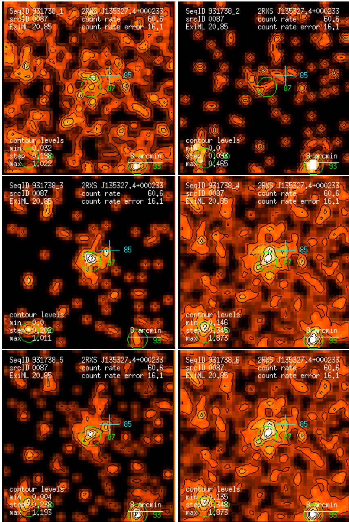
Figure 87: RASS 931738: detection 0087: band rate images, Gaussian filter: (1) PSPC channels 11 – 41, (2) 52 – 90, (3) 91 – 201, (4) 11 – 235, (5) 52 – 201, (6) 11 – 201. Broad band rates in counts/ks. Band rate contour levels in counts/ks/arcmin 2 .
