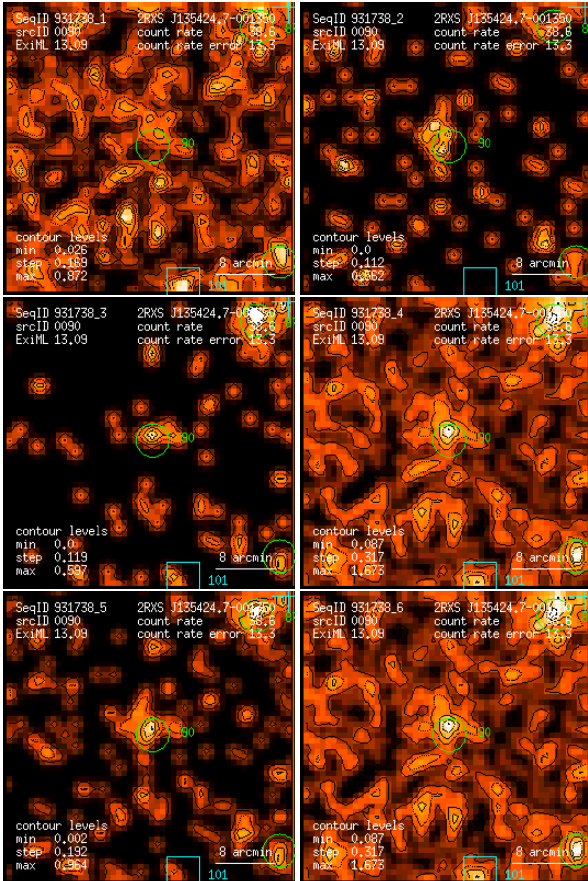
Figure 90: RASS 931738: detection 0090: band rate images, Gaussian filter: (1) PSPC channels 11 – 41, (2) 52 – 90, (3) 91 – 201, (4) 11 – 235, (5) 52 – 201, (6) 11 – 201. Broad band rates in counts/ks. Band rate contour levels in counts/ks/arcmin 2 .
