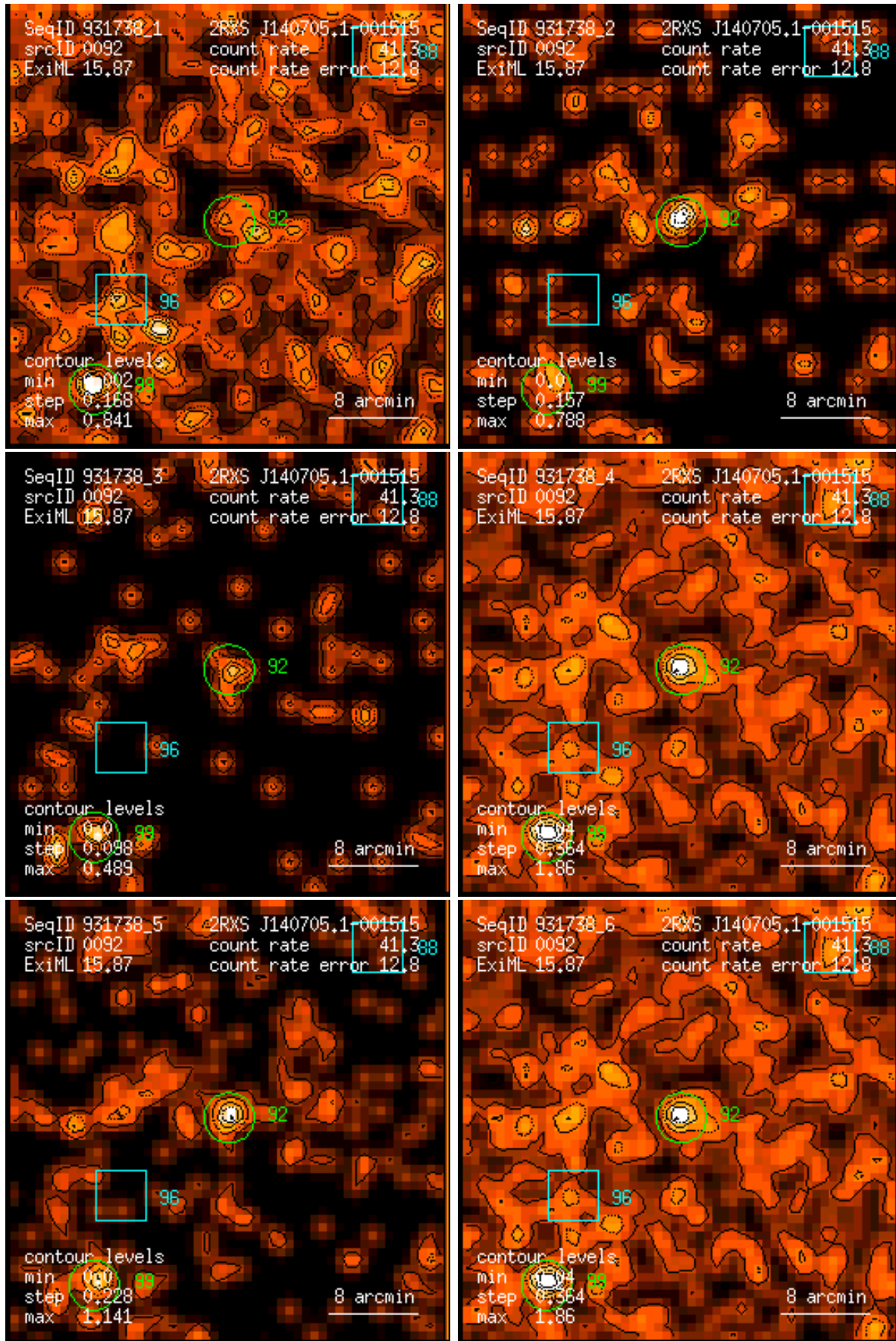
Figure 92: RASS 931738: detection 0092: band rate images, Gaussian filter: (1) PSPC channels 11 – 41, (2) 52 – 90, (3) 91 – 201, (4) 11 – 235, (5) 52 – 201, (6) 11 – 201. Broad band rates in counts/ks. Band rate contour levels in counts/ks/arcmin 2 .
