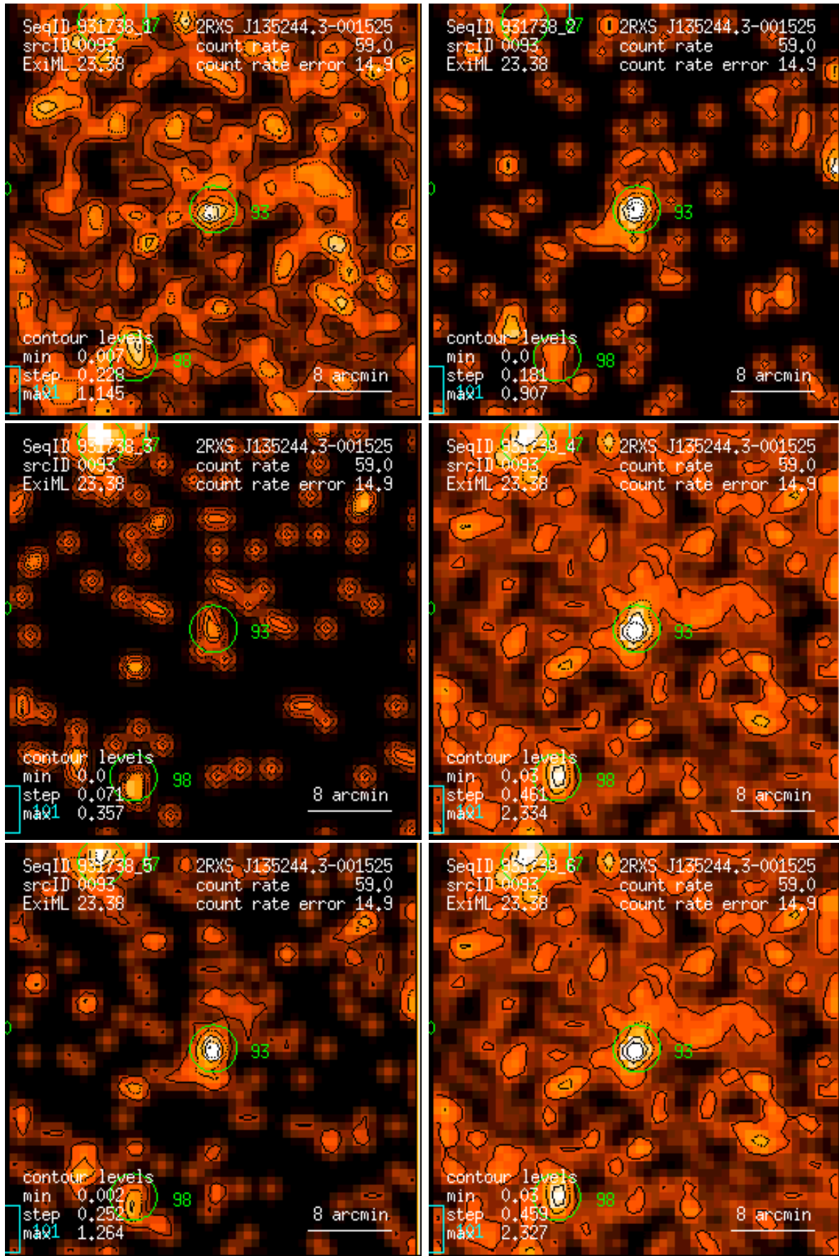
Figure 93: RASS 931738: detection 0093: band rate images, Gaussian filter: (1) PSPC channels 11 – 41, (2) 52 – 90, (3) 91 – 201, (4) 11 – 235, (5) 52 – 201, (6) 11 – 201. Broad band rates in counts/ks. Band rate contour levels in counts/ks/arcmin 2 .
