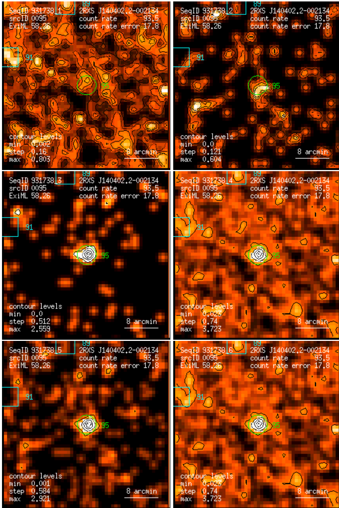
Figure 95: RASS 931738: detection 0095: band rate images, Gaussian filter: (1) PSPC channels 11 – 41, (2) 52 – 90, (3) 91 – 201, (4) 11 – 235, (5) 52 – 201, (6) 11 – 201. Broad band rates in counts/ks. Band rate contour levels in counts/ks/arcmin 2 .
