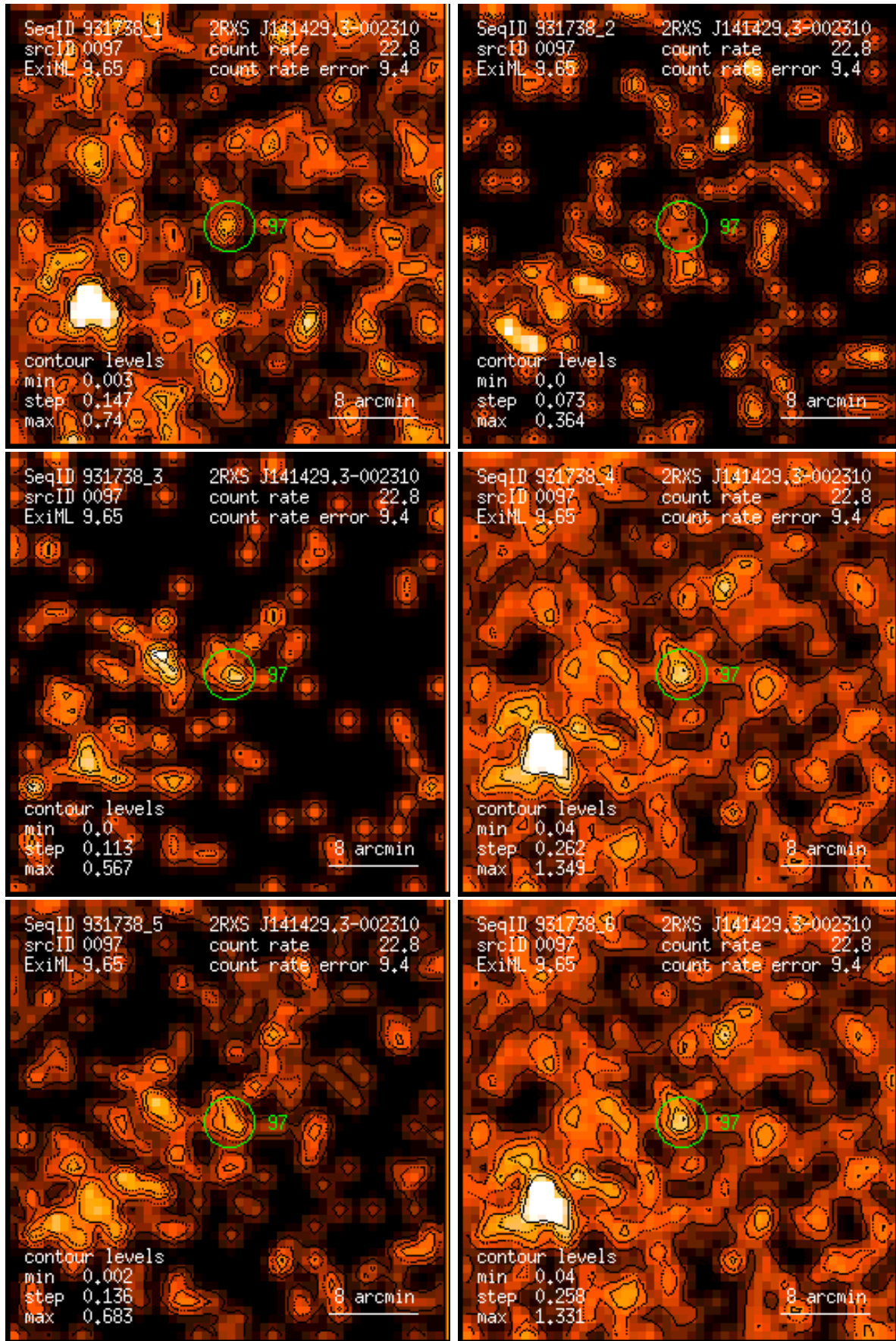
Figure 97: RASS 931738: detection 0097: band rate images, Gaussian filter: (1) PSPC channels 11 – 41, (2) 52 – 90, (3) 91 – 201, (4) 11 – 235, (5) 52 – 201, (6) 11 – 201. Broad band rates in counts/ks. Band rate contour levels in counts/ks/arcmin 2 .
