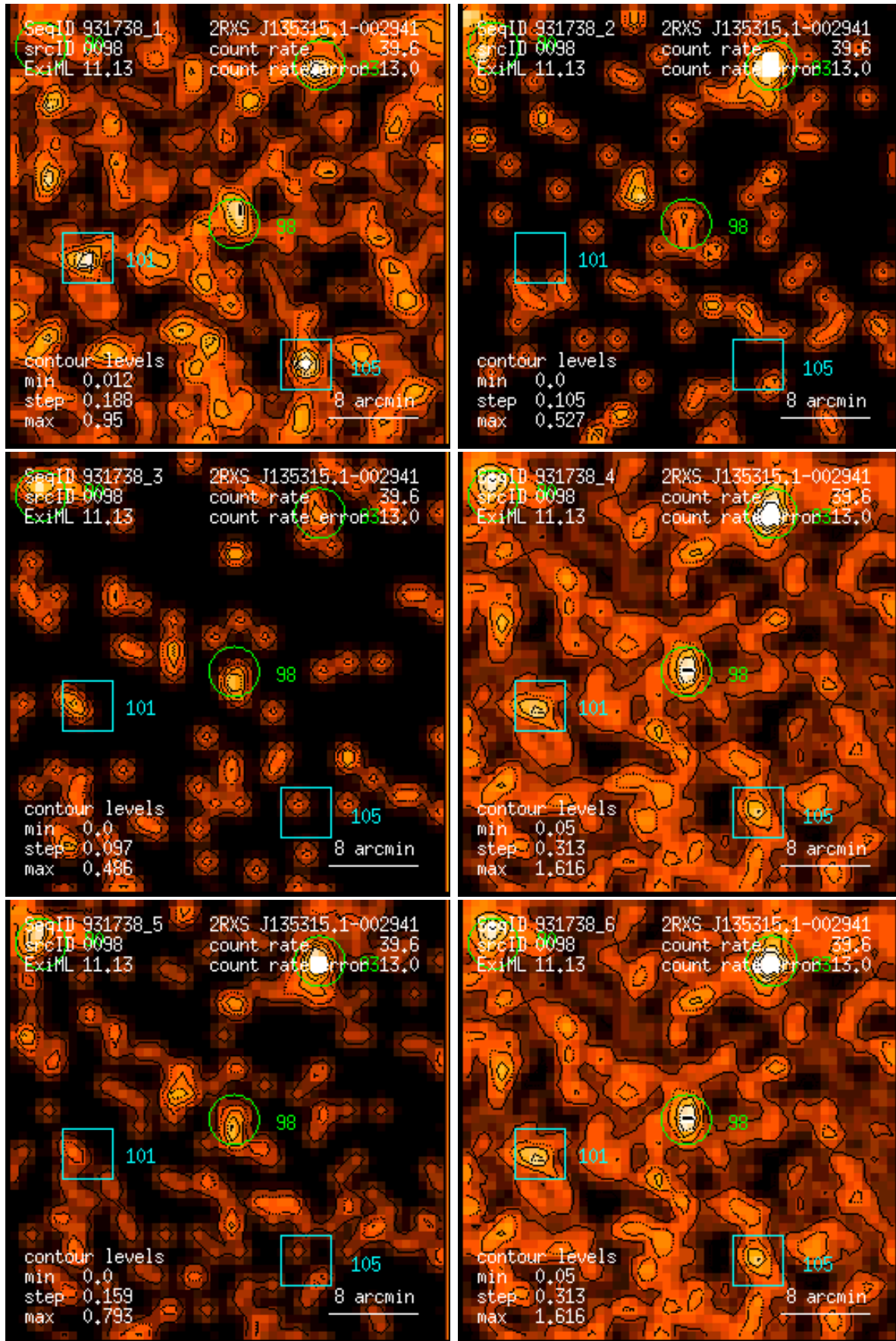
Figure 98: RASS 931738: detection 0098: band rate images, Gaussian filter: (1) PSPC channels 11 – 41, (2) 52 – 90, (3) 91 – 201, (4) 11 – 235, (5) 52 – 201, (6) 11 – 201. Broad band rates in counts/ks. Band rate contour levels in counts/ks/arcmin 2 .
