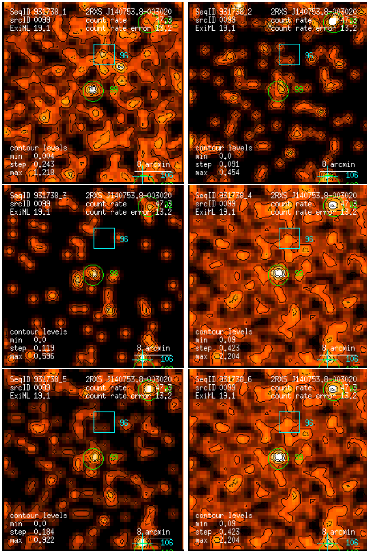
Figure 99: RASS 931738: detection 0099: band rate images, Gaussian filter: (1) PSPC channels 11 – 41, (2) 52 – 90, (3) 91 – 201, (4) 11 – 235, (5) 52 – 201, (6) 11 – 201. Broad band rates in counts/ks. Band rate contour levels in counts/ks/arcmin 2 .
